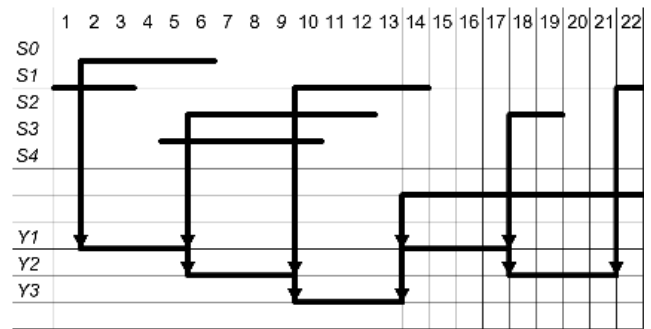
Fig. 2 Example of the cyclogram used in automatic control mode of galvanic line, where: S0: system activation; S1: traverse auto-operator in the upper position; S2: traverse auto-operator in the lower position; S3: suspension with details grasped by the auto-operator; S4: auto-operator over a given technological position and output signals Y1: lowering the traverse of the auto-operator; Y2: raising the traverse of the auto-operator; Y3: move the auto operator.
