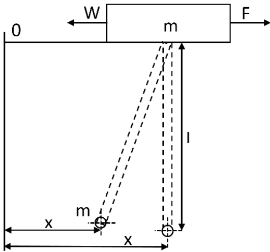
Fig. 7 Two-mass model of the mechanism of the automatic manipulator for galvanic line.
