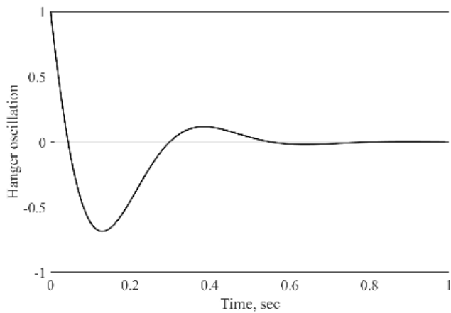
Fig. 10 Graph of a dynamic system by oscillations of the hanger with optimal controller by eliminated modeling.
