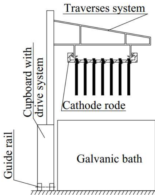
Fig. 4 Sketch of the console robot-manipulator.
