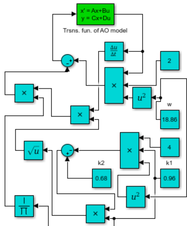
Fig. 9 Structural scheme of the system with the optimal controller by accelerating modeling.
