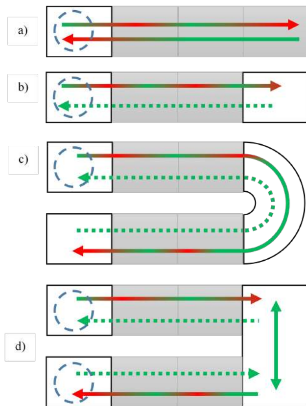
Fig. 1 Types of galvanic lines, where (a): linear galvanic line with the same initial and final position of auto-operator; (b): linear galvanic line with the different initial and final position of auto-operator; (c): two-row oval galvanic line; (d): two-row square galvanic line.
