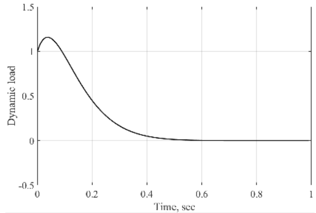
Fig. 13 Graph of a dynamic system by dynamic load of motor-drive with the optimal controller by accelerating modeling.
