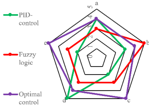
Fig. 6 Comparison of types of control, with a: frequency of use; b: control system reconfiguration speed when changing process conditions; c: the possibility of accounting for disturbances; d: ease of implementation; e: the ability to control the speed of movement of the auto operator.
