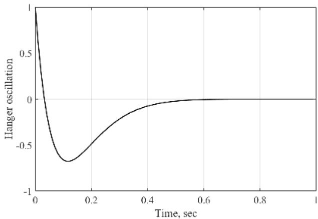
Fig. 11 Graph of a dynamic system by oscillations of the hanger with optimal controller by accelerating modeling.
