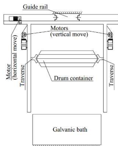
Fig. 3 Sketch of the telpher robot-manipulator.
