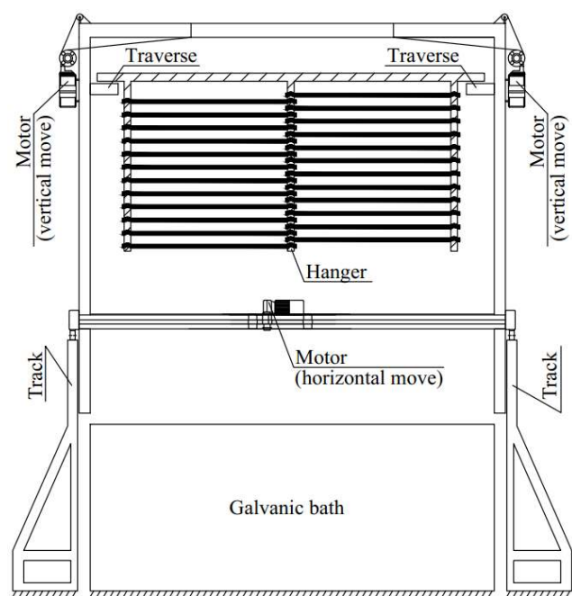
Fig. 5 Sketch of the portal robot-manipulator.
