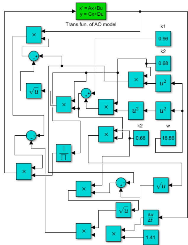
Fig. 8 Structural scheme of the system with the optimal controller by eliminated modeling.
