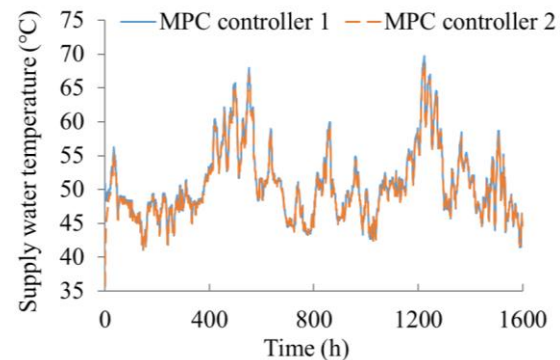
Fig. 12. Supply water temperature optimized by MPC controller 1 and MPC controller 2.
