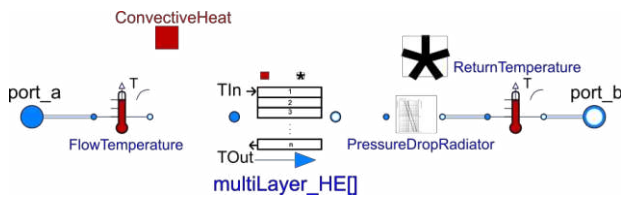
(a) Radiator block developed in Modelica.
