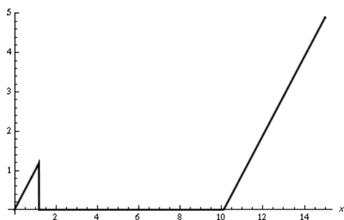
FIG. 10. Optimal policy f^{\pi^*}(x)
