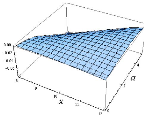
FIG. 13. a + \tilde{V}(x - a; b^*) - V(x; b^*) , large x
