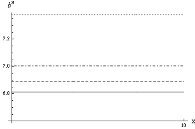
FIG. 1. V(x; b^n) for n = 1, 10, 50, 1000
