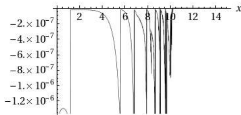
FIG. 11. TV(x; \pi^*) - V(x; \pi^*)
