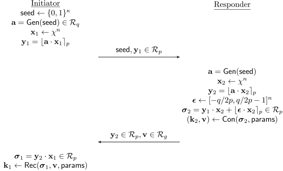
Figure 14: RLWR-based key exchange from KC
