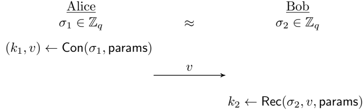
Figure 2: Brief depiction of KC, where k_1, k_2 \in \mathbb{Z}_m , v \in \mathbb{Z}_g and |\sigma_1 - \sigma_2|_q \leq d .
