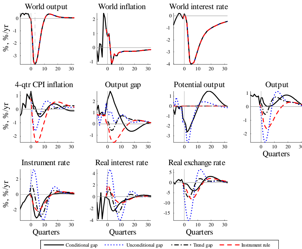
Figure 5.2: Difference between unconditional and conditional projections in 2008:3 for optimal policy with different output gaps ( \lambda_y = 1.1, \lambda_{\Delta i} = 0.37 )
