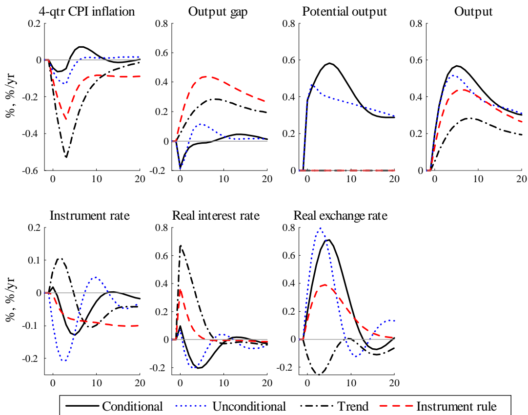
Figure 4.1: Impulse responses to a (one-standard deviation) stationary technology shock under optimal policy for different output gaps and under the instrument rule
