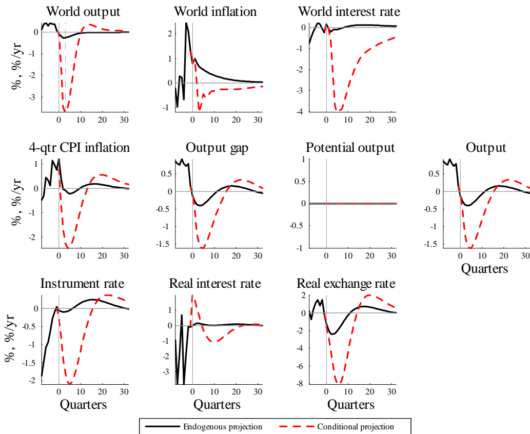
Figure 5.1: Projections in 2008:3 for the instrument rule
