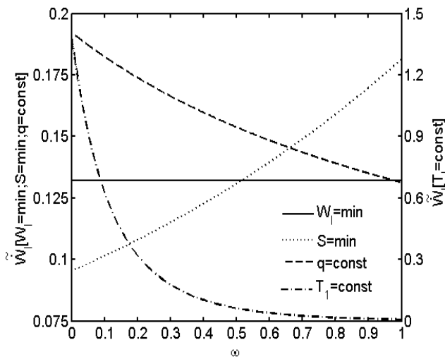
FIG. 4: Dependence of the dimensionless rate of lost available work \dot{\tilde{W}}_l on the dimensionless time \omega in case of the Dulong-Petit heat transfer law
