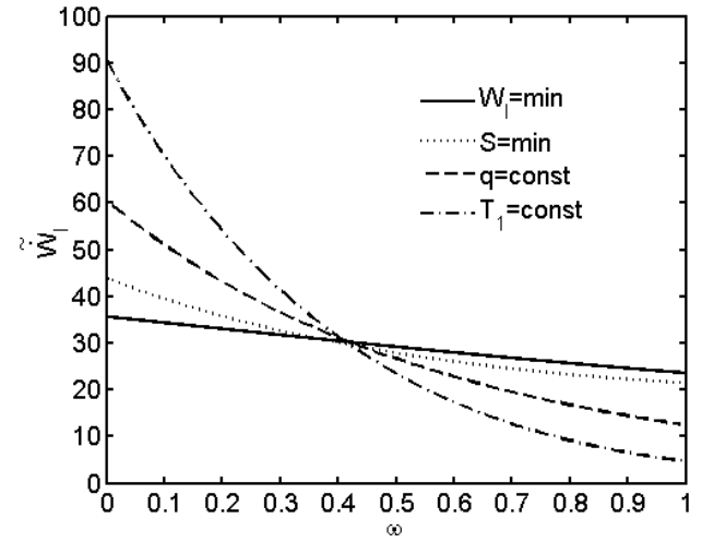
FIG. 8: Dependence of the dimensionless rate of lost available work \tilde{W}_l on the dimensionless time \omega in case of the heat transfer law q \propto (\Delta(T^4))^{1.25}
