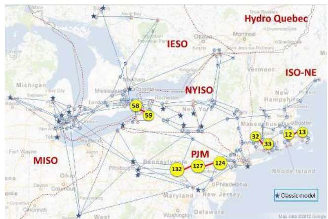
Fig. 4. Map of the NPCC 48-machine 140-bus system. The stars indicates generators with classical model and the transmission lines with highest line flow and their buses are highlighted.
