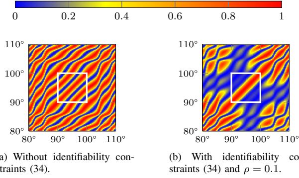
Fig. 3. Colormap of left hand side of (34) versus \theta and \theta' when employing AoD-AoA-optimal precoders. The Tx and the Rx have, each, a 30-antennas uniform linear array (ULA) [38]. The number of training sequences M = 4 and the rank of \mathbf{X} is 4. It is known a priori that the AoD lies in the interval \mathcal{R}_{\text{Tx}} = [90^\circ, 100^\circ] . The white square indicates the region \mathcal{R}_{\text{Tx}} \times \mathcal{R}_{\text{Tx}} .
