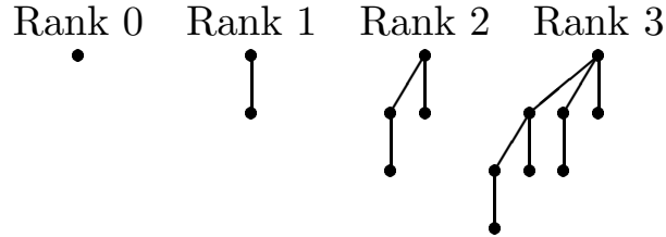
Figure 2: Binomial trees of ranks 0–3.
