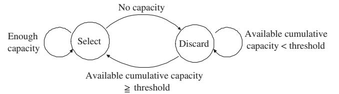
Fig. 6. State transition diagram specifying the quality adaptation mechanism.
