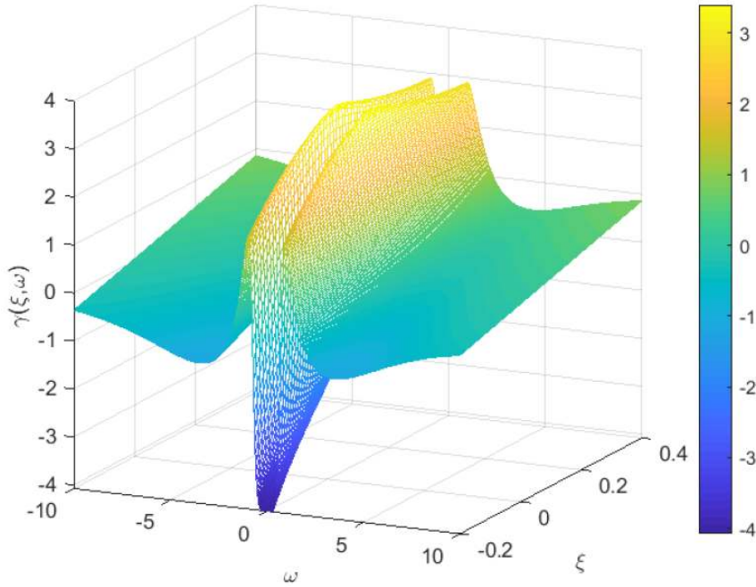
FIG. 5.2. 3D illustration of \gamma(\xi, \omega) .
