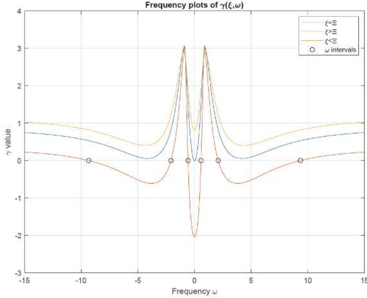
FIG. 5.1. Three frequency plots for the cases \xi smaller, equal and larger than \Xi
