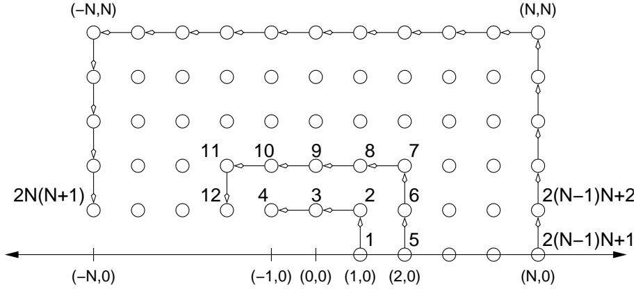
FIG 3. The construction of the ordering mapping \sigma : \mathbb{Z}_V^2 \mapsto \mathbb{Z}^+ . The circles represent points in \mathbb{Z}_V^2 . The paired numbers in parenthesis are co-ordinates of points; the single numbers show the ordering of points w.r.t. \sigma(\cdot) . For example, \sigma((2, 0)) = 5 , \sigma((2, 2)) = 7 .
