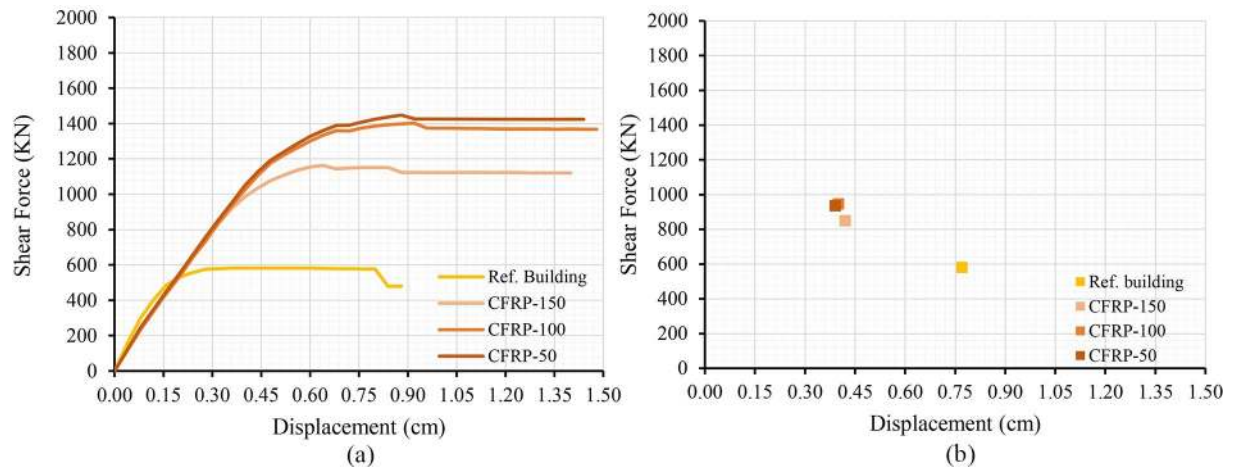
Fig 8. Capacity curves (a) and performance points (b) of the models adding CFRP bands varying the band spacing.
