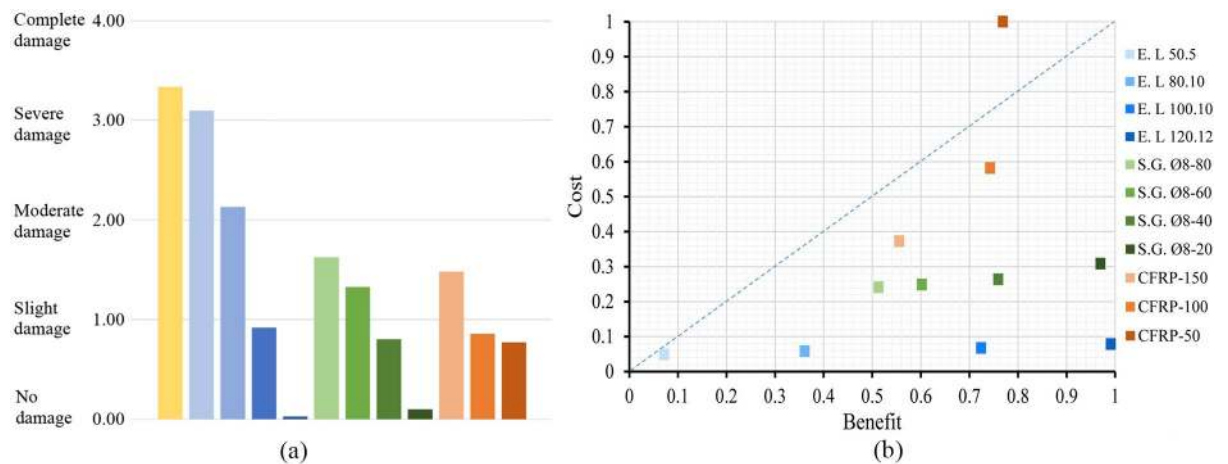
Fig 11. DI for each retrofitting solution (a) and cost-benefit index (b).
