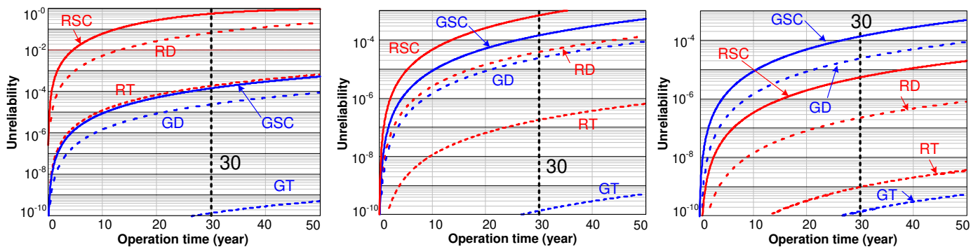
Fig. 9. Unreliability from power devices to power converter with the same design of the grid-side converter. (a) Two modules in rotor-side converter. (b) Three modules in rotor-side converter. (c) Four modules in rotor-side converter.
