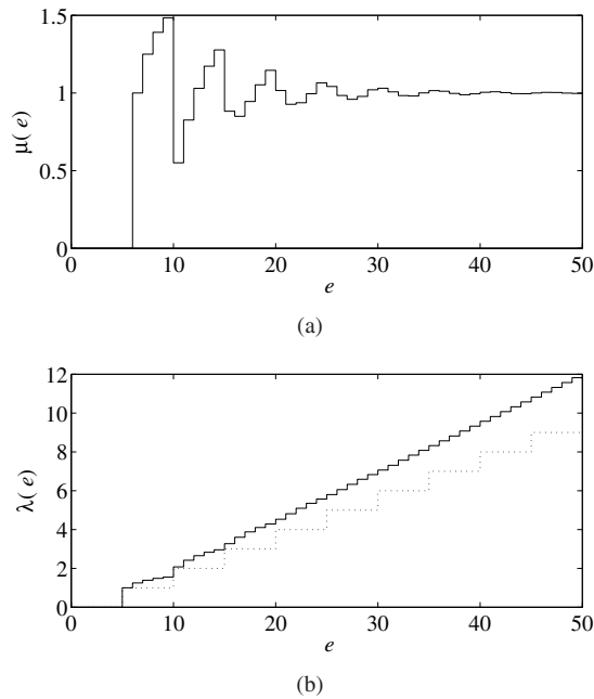
Fig. 2: The decision threshold (a) and the expected importance sum (b) (continuous line) as a function of the available energy. A uniform importance distribution U(0, 2) with E_T = 4 and E_R = 1 is assumed. The stepwise function (dotted line) reflects the behavior of a non-selective transmitter, which transmits any message whatever its importance value is.
