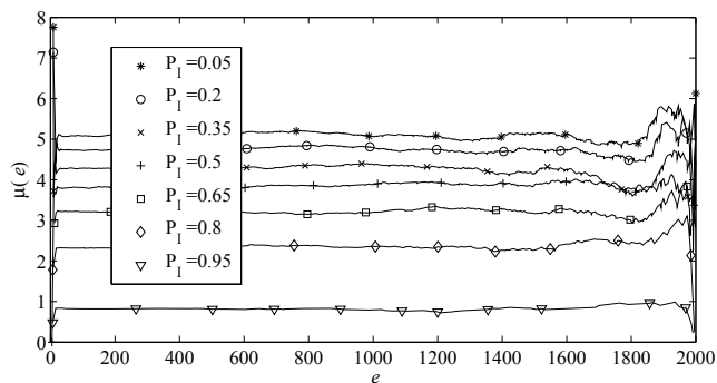
Fig. 9: Threshold evolution regarding to the remaining battery level e in an isolated AT sensor node for a uniform importance distribution U(0, 10) . Different frequencies of being in idle state have been considered in a single run.
