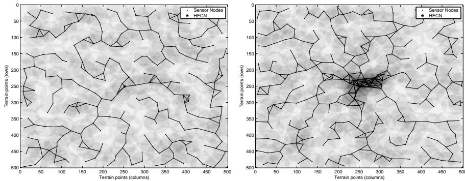
Figure 2: Example solutions obtained with MOEA: minimum number of nodes (left), minimum energy spent (right).
