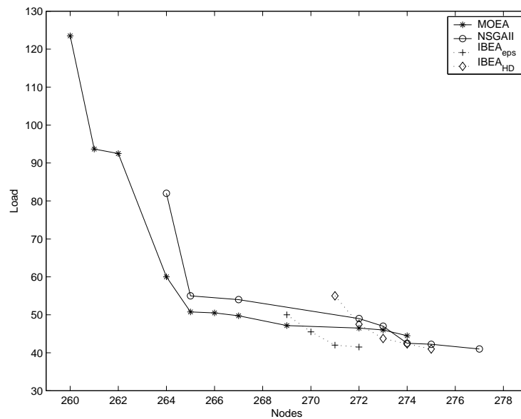
Figure 3: Best fronts obtained by the algorithms MOEA, NSGAII, IBEA ε and IBEA HD
