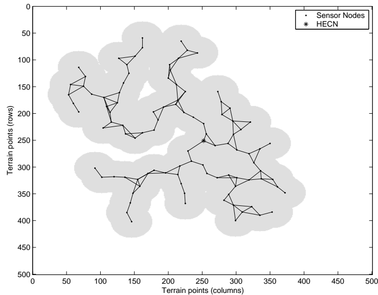
Figure 1: Wireless Sensor Network Example.
