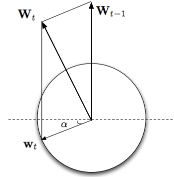
Figure 1: Illustration for the proof of the minimax strategy for the ball. We suppose that \mathbf{x}_t is aligned with \mathbf{W}_{t-1} and depict the plane spanned by \mathbf{W}_{t-1} and \mathbf{w}_t . We assume that \mathbf{w}_t has angle \alpha with the line perpendicular to \mathbf{W}_{t-1} and show that \alpha = 0 is optimal.
