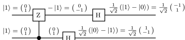
Fig. 1. Quantum circuit
