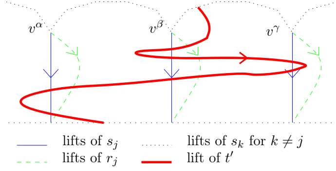
Figure 8: A view of \tilde{\mathcal{M}}(s, j, \tilde{t}') , the lifts of r_j , s_j , and the lift \tilde{t}' . Here, [r + s/t'] = \bar{r}_j^\beta \bar{s}_j^\beta s_j^\beta r_j^\beta s_j^\gamma \bar{s}_j^\gamma \bar{r}_j^\beta \bar{s}_j^\beta \bar{r}_j^\alpha \bar{s}_j^\alpha s_j^\alpha r_j^\alpha .
