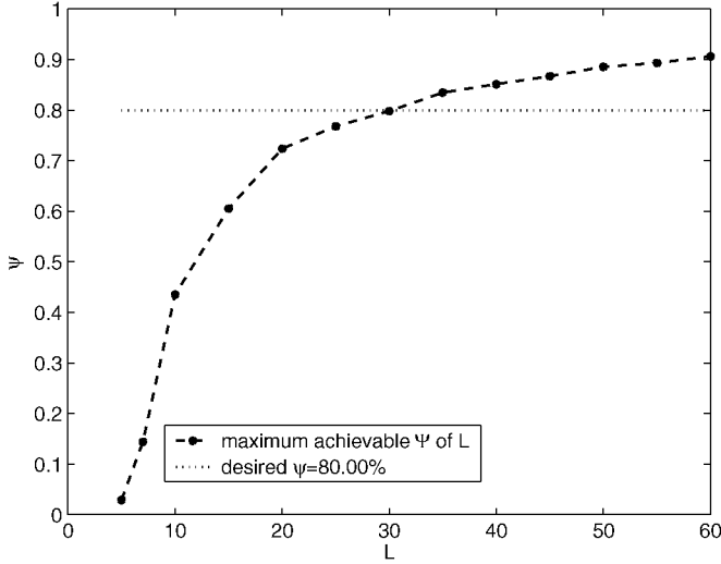
Fig. 6. Maximum achievable NESP \psi versus L under the tighter mask S_{TmT}(f) .
