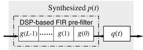
Fig. 1. DSP-based UWB pulse design.
