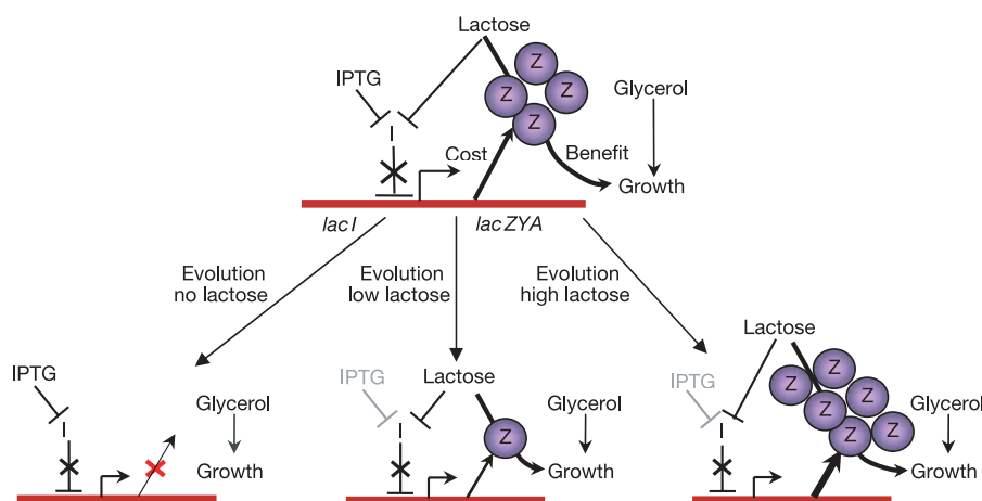
Figure 1 | The lac operon of E. coli and the experimental design in the present study. The lac operon encodes the enzyme LacZ, denoted Z, which uses the sugar lactose, L, to increase growth rate. In the experiments, we consider environments with constant concentrations of lactose. The repressor of the lac system LacI, denoted I, was deactivated by the presence of lactose. To examine evolution at zero lactose under the same conditions, we added the non-metabolized inducer IPTG, which also deactivates LacI, and glycerol as an additional carbon source, in all cases. Measurements on
