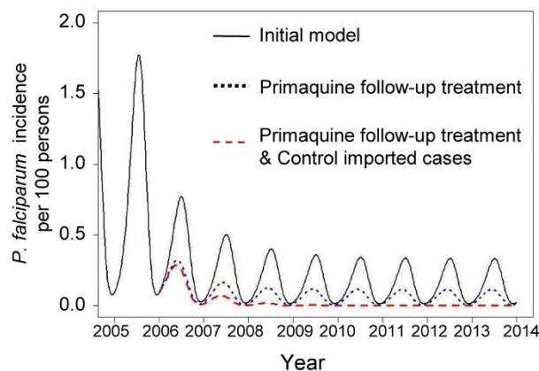
Figure 7 Estimated P. falciparum malaria incidence for different control policies. Solid line represents the incidence estimated by the initial model when the standard drug regimen (2-day ACTs and Primaquine at day 2) was used (solid line). The incidence significantly decreased when the timing of primaquine administration was shifted to the eighth day after initial attack (short-dashed line). The elimination of malaria transmission can be reached when the combination of both primaquine follow-up treatment and control of imported asymptomatic cases was implemented (long-dashed line).
