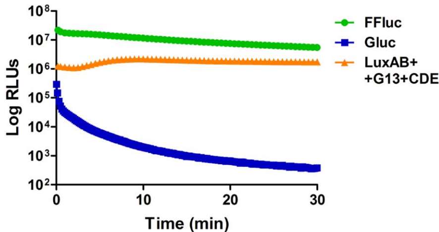
Figure 7. Light production from FFluc and Lux is stable, whereas the signal from Gluc rapidly dissipates. Luminescence (given as relative light units [RLUs]) was measured every 10 s for gluc -expressing M. smegmatis and every 30 s for ffluc - or lux -expressing M. smegmatis , over a 30 min period. The integration times used were 0.1 s, 5 s and 10 s for Gluc, FFluc and Lux respectively. At time point 0 min, 470 \mu M luciferin or 40 \mu M coelenterazine were added to FFluc- and Gluc-producing M. smegmatis respectively. Two independent cultures were used for FFluc and Lux, and three for Gluc. Each culture was measured in duplicate and the means and standard deviations (smaller than symbols) are plotted. doi:10.1371/journal.pone.0010777.g007
