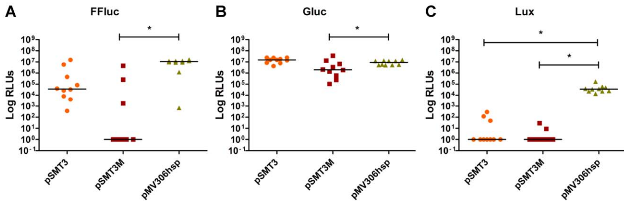
Figure 1. Expression from an integrating vector results in the highest and most stable bioluminescent signal. To study the effect of copy number on light production each reporter was cloned into standard (pSMT3), high (pSMT3M), and single copy number (pMV306hsp) vectors. Luminescence was measured for 10 independent M. smegmatis transformants each carrying the FFluc (a), Gluc (b) and Lux (c) constructs. Results are given as relative light units (RLUs) and are corrected for the background. Overall differences between groups were assessed using the Kruskal–Wallis non-parametric test with differences between subgroups assessed by Dunn’s multiple comparisons test and those found to be significant ( p < 0.01 ) are indicated with *. doi:10.1371/journal.pone.0010777.g001
