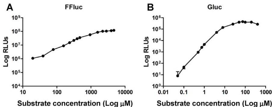
Figure 6. Bioluminescence correlates with substrate concentration at low concentrations. Luminescence (given as relative light units [RLUs]) of M. smegmatis pMVhsp+FFluc (a) and M. smegmatis pMVhsp+Gluc (b) was measured with integration times of 5 s and 0.1 s respectively. The substrate concentrations assayed ranged from 20 to 4710 \mu\text{M} luciferin for FFluc, and from 0.05 to 400 \mu\text{M} coelenterazine for Gluc. Means and standard deviations (smaller than symbols) of six replicates are shown. doi:10.1371/journal.pone.0010777.g006
