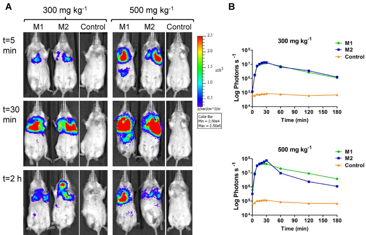
Figure 10. Kinetics of FFluc activity in M. smegmatis infected mice after intraperitoneal injection of luciferin. Mice were endotracheally inoculated with 1.4 \times 10^7 CFU of M. smegmatis pMV306hsp+FFlucWT [two representative mice (M1 and M2) out of four are shown] or with 6.8 \times 10^6 CFU of M. smegmatis pMV306hsp (control). 300 mg kg -1 or 500 mg kg -1 luciferin intraperitoneal was given 24 h post-inoculation and images were acquired at time points 0 (immediately after substrate administration), 5, 10, 15, 20, 25, 30, 60, 120 and 180 min. (a) Images were obtained using an IVIS Spectrum and are displayed as pseudocolour images of peak bioluminescence (given as photons s -1 cm -2 steradian [sr -1 ]), with variations in colour representing light intensity at a given location. Mice injected with 300 mg kg -1 luciferin were imaged with an integration time of 1 min, whereas those that received 500 mg kg -1 luciferin were imaged for 10 s to avoid saturation of the image. Three representative time points are shown. (b) Bioluminescence (given as photons s -1 ) in the thorax was quantified for each time point using the region of interest tool in the Living Image software program.
