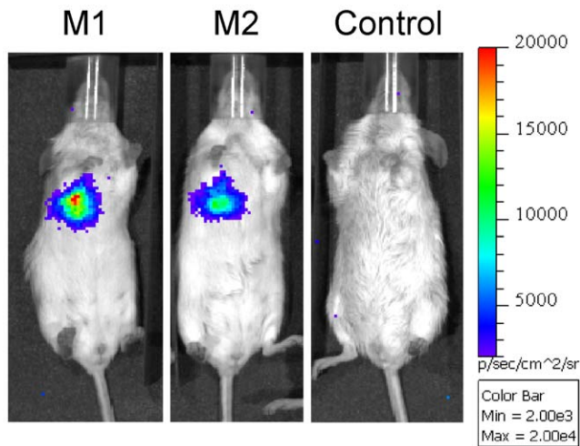
Figure 13. BLI of lux -expressing M. smegmatis . Mice were inoculated endotracheally with M. smegmatis pMV306hsp+Lux-AB+G13+CDE [ 7.9 \times 10^6 CFU, two mice (M1 and M2) out of four are shown] or M. smegmatis pMV306hsp ( 6.8 \times 10^6 CFU, control) and imaged 24 h post-inoculation. Images were obtained using an IVIS Spectrum and are displayed as pseudocolor images of peak bioluminescence (given as photons s^{-1} cm^{-2} sr^{-1} ), with variations in colour representing light intensity at a given location. Mice were imaged with an integration time of 5 min. doi:10.1371/journal.pone.0010777.g013
