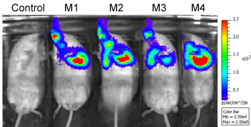
Figure 14. BLI of ffluc -expressing M. tuberculosis . Mice were inoculated endotracheally with 5 \times 10^6 CFU of either wild-type M. tuberculosis (control) or FFluc-producing M. tuberculosis . 20 \mu l of 30 mg ml^{-1} luciferin was administered intranasally and mice were imaged 5–10 min after. Mice were contained in a large air-tight box for safety considerations. The image was obtained using an IVIS Spectrum and is displayed as a pseudocolor image of peak bioluminescence (given as photons s^{-1} cm^{-2} sr^{-1} ). Red represents the most intense light emission while blue correspond to the weakest signal. The colour bar indicates relative signal intensity. Mice were imaged with an integration time of 1 min. doi:10.1371/journal.pone.0010777.g014
