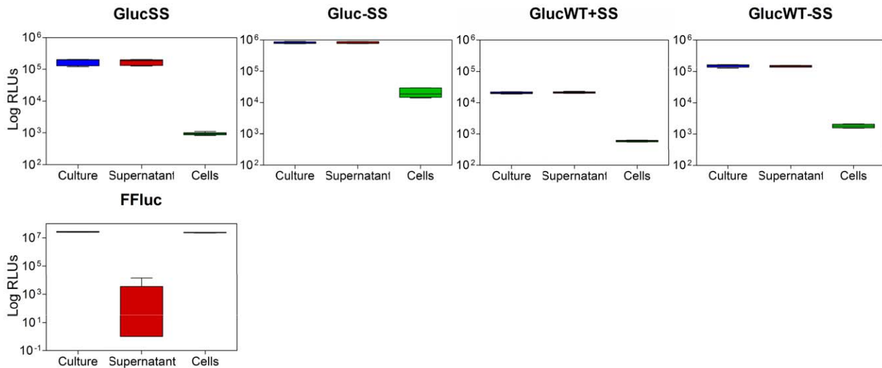
Figure 9. Gaussia luciferase is secreted from mycobacterial cells. Luminescence (given as relative light units [RLUs]) was measured in culture, supernatant and cell samples of M. smegmatis producing Gluca Mycobacterium optimised with (GlucSS) or without (Gluc) signal peptide, Gluc wild-type with (GlucWT+SS) or without (GlucWT-SS) signal peptide, and FFluc as control. Assays were performed with three independent cultures and each culture was measured in duplicate. As the data was not normally distributed, median values are displayed (bar) with inter-quartile ranges (box), and highest and lowest values (whiskers). doi:10.1371/journal.pone.0010777.g009
