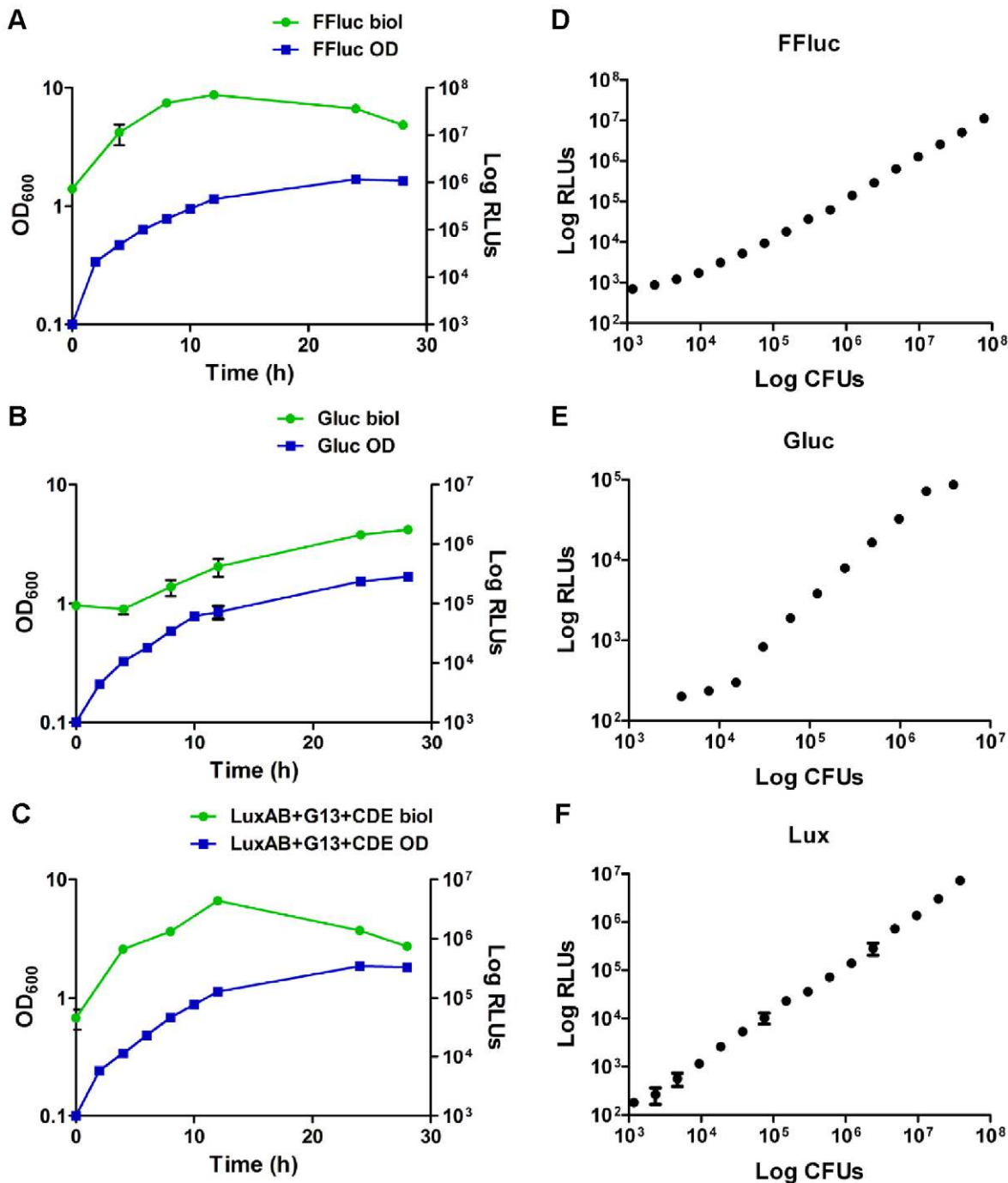
Figure 8. Bioluminescence correlates with cell density during exponential growth in vitro . Cultures of M. smegmatis pMVhsp+FFluc (a), pMVhsp+Gluc (b) and pMVhsp+Lux (c) were inoculated to an optical density (OD) at 600 nm of 0.1 and the OD and the luminescence [given as relative light units (RLUs)] measured over 28 h. The luminescence was measured with integration times of 5, 0.1, and 10 s respectively, and substrate concentrations of 470 \mu M luciferin for FFluc and 40 \mu M coelenterazine for Gluc. The values represented correspond to the means of two independent cultures measured in triplicate. The error bars indicate standard deviations. A near linear relationship was found between bioluminescence [given as RLUs] and colony counts (given as colony forming units [CFU]) for mid-log cultures of M. smegmatis pMVhsp+FFluc (d), pMVhsp+Gluc (e) and pMVhsp+Lux (f) using a plate luminometer. doi:10.1371/journal.pone.0010777.g008
