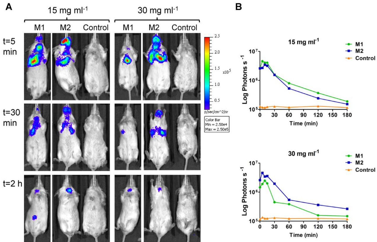
Figure 11. Kinetics of FFluc activity in M. smegmatis infected mice after intranasal administration of luciferin. Mice were endotracheally inoculated with 6.6 \times 10^6 CFU of M. smegmatis pMV306hsp+FFlucWT [two representative mice (M1 and M2) out of four are shown] or with 6.8 \times 10^6 CFU of M. smegmatis pMV306hsp as a control (one representative mouse out of two is shown). 20 \mu l of 15 mg ml -1 or 30 mg ml -1 luciferin intranasal was administered 24 h post-inoculation and mice were imaged 0, 5, 10, 15, 30, 60, 120 and 180 min after. (a) Images were obtained using an IVIS Spectrum and are displayed as pseudocolor images of peak bioluminescence (given as photons s -1 cm -2 sr -1 ). Red represents the most intense light emission while blue correspond to the weakest signal. The colour bar indicates relative signal intensity. Mice were imaged with an integration time of 30 s. Three representative time points are shown. (b) Signal intensity (given as photons s -1 ) in the lungs was quantified for each time point using the region of interest tool in the Living Image software program. doi:10.1371/journal.pone.0010777.g011
