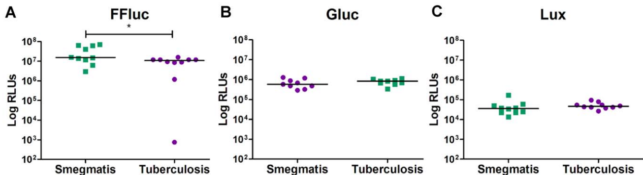
Figure 4. Bioluminescence levels in M. tuberculosis and M. smegmatis are comparable in vitro . Relative light units (RLUs) were measured in 10 M. smegmatis and 10 M. tuberculosis clones transformed with pMV306hsp+FFluc (a), pMV306hsp+Gluc (b) or pMV306hsp+Lux (c). Results are corrected for the background. Statistical significance was evaluated by the Mann-Whitney non-parametric test for Lux, and by unpaired t test for FFluc and Gluc (data normality passed) and those found to be significant ( p < 0.05 ) are indicated with *. doi:10.1371/journal.pone.0010777.g004
