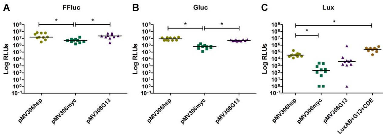
Figure 2. Expression of luciferases using promoters P_{hsp60} and P_{G13} leads to greater light production. Luminescence of M. smegmatis expressing ffluc (a), gluc (b) and lux (c) was assayed using P_{hsp60} , P_{myc} tetO, and P_{G13} in the integrating vector pMV306. Each dot represents a randomly selected transformant. Results are given as relative light units (RLUs) and are corrected for the background. Statistical significance was evaluated by the Kruskal–Wallis test with subgroup analysis performed by Dunn’s multiple comparison test and those found to be significant ( p < 0.05 ) are indicated with *. doi:10.1371/journal.pone.0010777.g002
