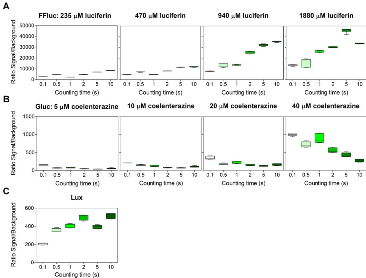
Figure 5. Signal:noise for FFluc and Lux increases with integration time, and decreases for Gluc. Luminescence was measured using six different integration times and four different substrate concentrations for M. smegmatis producing FFluc (a) and Gluc (b), or without substrate for Lux (c). The background luminescence was obtained from cultures of M. smegmatis with the empty pMV306hsp. Assays were performed with three independent mid-log cultures and each culture was measured in duplicate. As the data was not normally distributed, median values are displayed (bar) with inter-quartile ranges (box), and highest and lowest values (whiskers). doi:10.1371/journal.pone.0010777.g005
