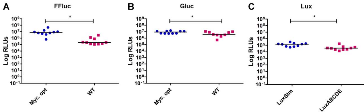
Figure 3. Codon optimisation increases bioluminescence in vitro . Relative light units (RLUs) were measured in 10 M. smegmatis clones transformed with a wild-type or a Mycobacterium optimised FFluc (a) or Gluc (b), or with a Gram positive or Streptomyces optimised Lux (c). In all cases pMV306hsp was used as backbone. Results are corrected for the background. Statistical significance was evaluated by the Mann-Whitney non-parametric test for FFluc and Lux, and by unpaired t test for Gluc (data normality passed) and those found to be significant ( p < 0.05 ) are indicated with *. doi:10.1371/journal.pone.0010777.g003
