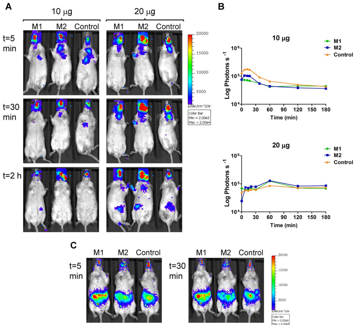
Figure 12. BLI of gluc -expressing M. smegmatis . Mice were endotracheally inoculated with 3.32 \times 10^6 CFU of M. smegmatis pMV306hsp+Gluc [two representative mice (M1 and M2) out of three are shown,] or with 1.58 \times 10^7 CFU of M. smegmatis pMV306hsp as a control (one out of two mice is shown). 10 µg of coelenterazine intranasal was administered 24 h post-inoculation and mice were imaged at time points 0, 5, 10, 15, 30, 60, 120 and 180 min. (a) Images were obtained using an IVIS Spectrum and are displayed as pseudocolor images of peak bioluminescence (given as photons s^{-1} cm^{-2} sr^{-1} ), with variations in colour representing light intensity at a given location. Integration time was 5 min. (b) Bioluminescence (given as photons s^{-1} ) was quantified using the Living image software. (c) 10 µg of coelenterazine was given intraperitoneally to the same mice 5 h post-intranasal coelenterazine. Mice were imaged 0, 5, 10, 15, 20, 25 and 30 min post-intraperitoneal coelenterazine with integration times of 3 min. doi:10.1371/journal.pone.0010777.g012
