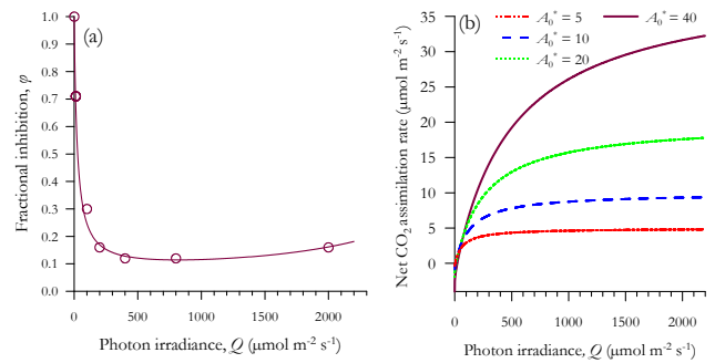
Fig. A1. Key features of the model. (a) Inhibition of leaf respiration in the light (Eq. A6); (b) Predicted variations net CO 2 assimilation rates for a range of leaf photosynthetic capacities (expressed as a maximum CO 2 assimilation rate in the absence of dark respiration, A_0^* , with units of \mu\text{mol m}^{-2} \text{s}^{-1} ) including an allowance for inhibition of leaf respiration in the light according to Eq. (A1) with R_z from Eq. (A6) and with \phi=0.008 \text{ mol CO}_2 \text{ mol}^{-1} \text{ quanta} ).
