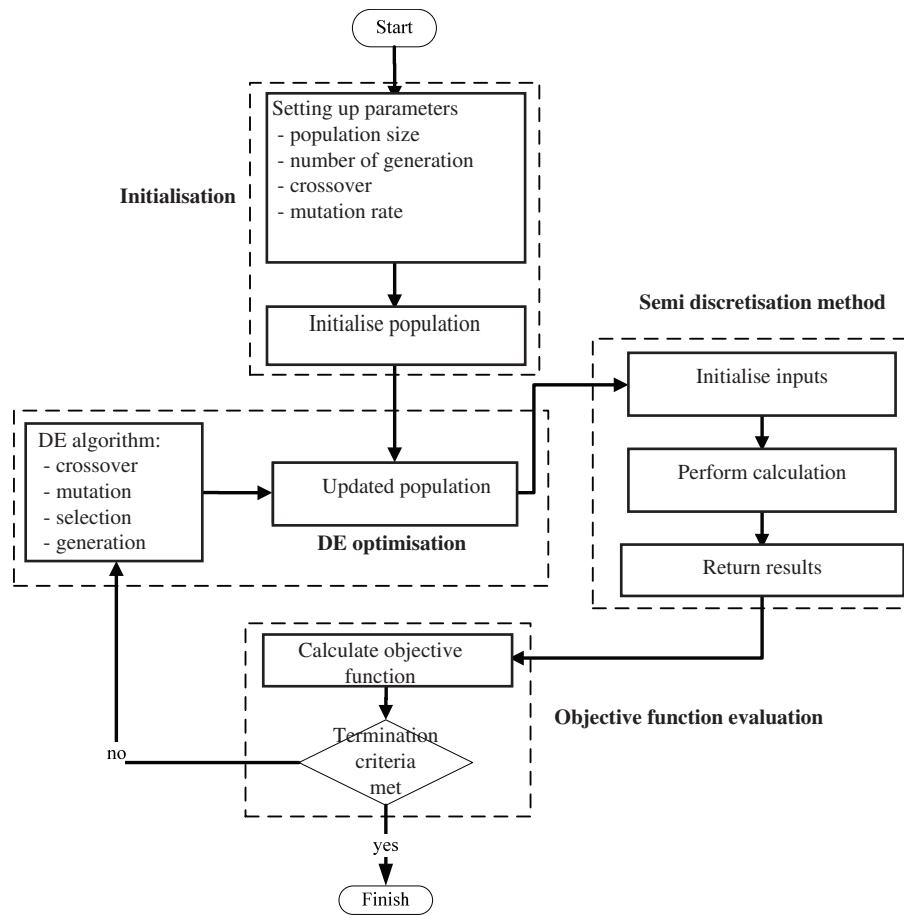
Figure 6: Optimisation methodology
