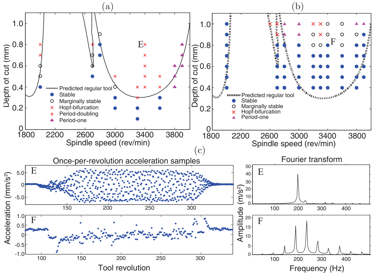
Figure 8: Analysis of experimental results. (a) Predicted and experimental stability of regular tool; (b) predicted and experimental stability of optimised variable helix tool; (c) Analysis of labelled data points E and F.
