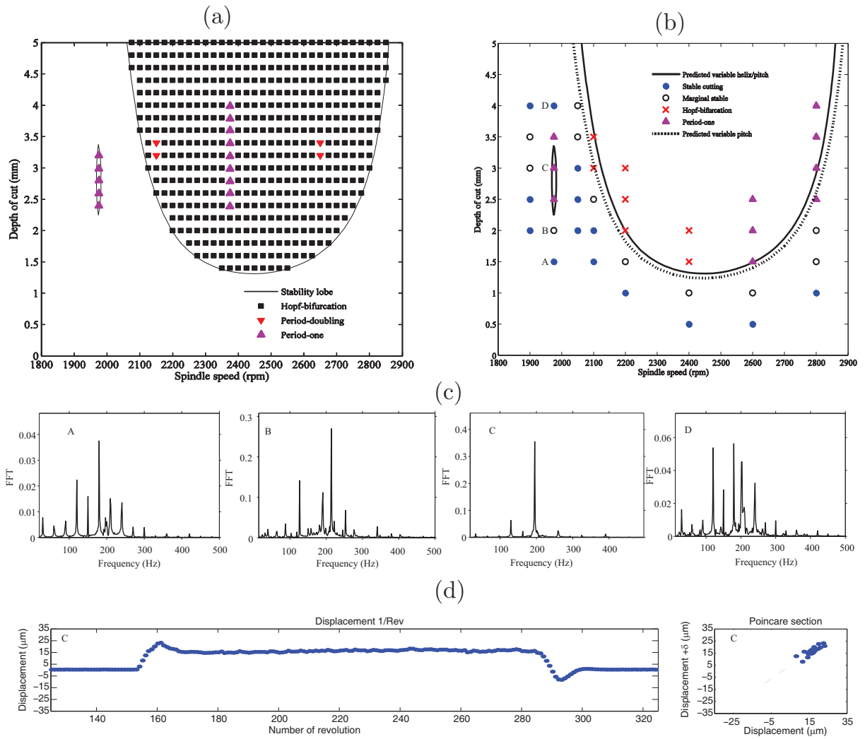
Figure 5: Experimental validation of the semi-discretisation method. (a) prediction; (b) experimental results with predicted stability boundary shown superimposed; (c) frequency-domain analysis for cases labelled A to D in (b) - note the different scales for each axis; (d) once/revolution samples and Poincaré section for case C.
