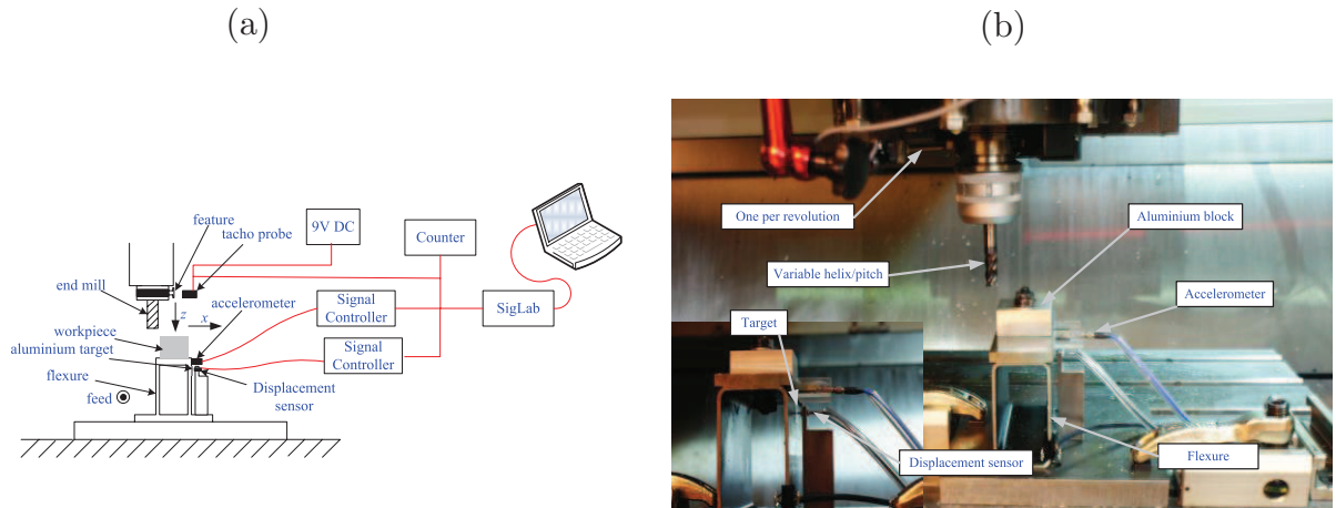
Figure 4: Experimental setup. (a) Schematic; (b) photograph.
