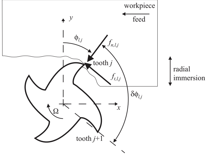
Figure 2: Schematic representation of cutting forces during milling
