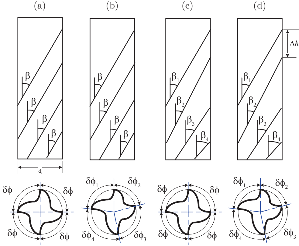
Figure 1: Variable pitch tool geometry for a 4 flute tool. (a) Regular tool - uniform pitch, uniform helix; (b) Variable pitch tool; (c) Variable helix tool - special case with regular pitch at the tool tip; (d) Variable helix tool
