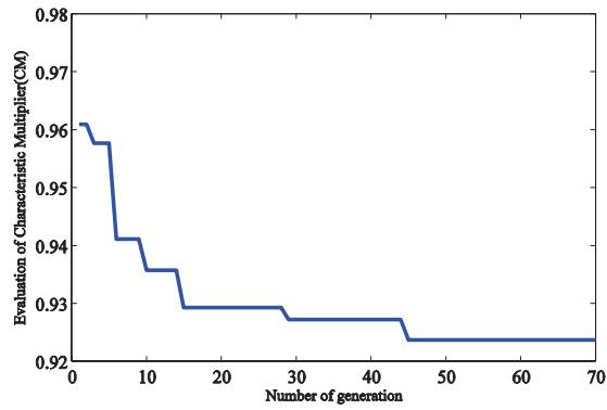
Figure 7: Optimisation results - evaluated objective function for increasing number of generations.
