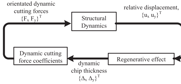
Figure 3: Block diagram of forces and displacements during milling
