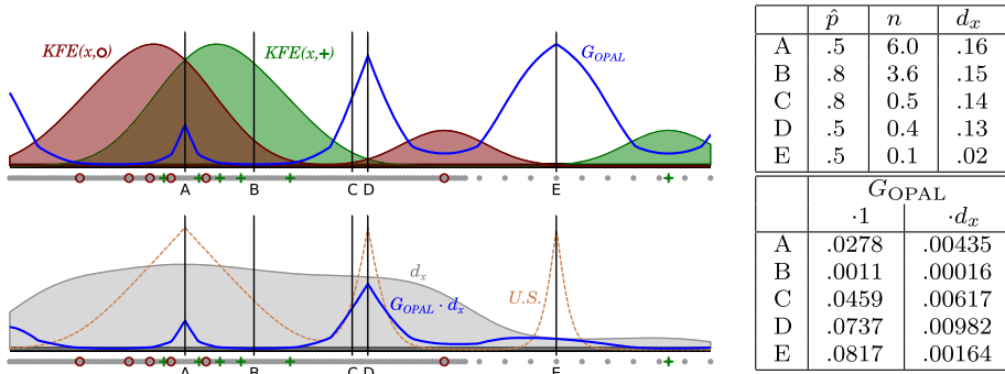
Fig. 2 Visualisation of G_{OPAL} -values for \tau = 0.5 on a one-dimensional dataset with labelled (red resp. green dots) and unlabelled (grey dots) data points. The upper plot shows the kernel frequency estimates (KFE) for each class and the corresponding G_{OPAL} -value (blue curve). The lower plot shows the density (grey area) and the density-weighted G_{OPAL} -values (blue curve). Additionally, the negative confidence values from the Uncertainty Sampling approach are plotted for comparison. For exemplary data points (A–E) the corresponding label statistics and the unweighted ( \cdot 1 ) and density weighted ( \cdot d_x ) G_{OPAL} -values are given in the tables
