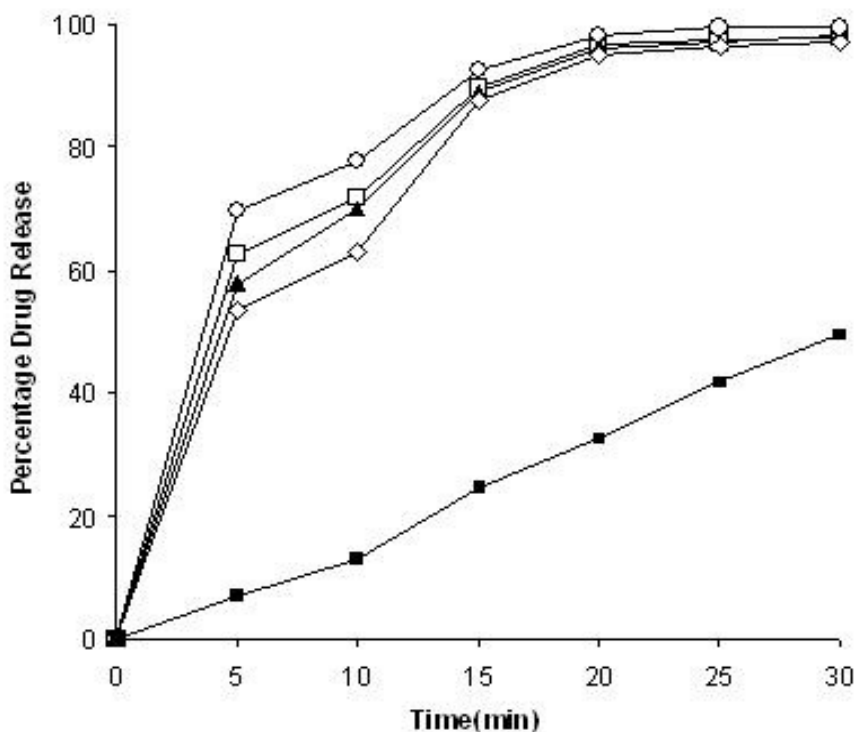
Figure 2: Drug release profile of formulations F1 - F4 and conventional meloxicam tablet in phosphate buffer (pH 6.41). (□— F1; ▲— F2; ◇— F3; ○— F4; ■— conventional meloxicam tablet)
