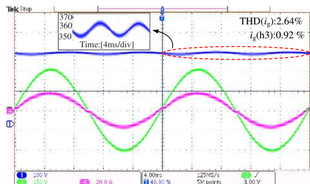
Fig. 21. Steady-state waveforms with the traditional PI + bulky capacitor method.
