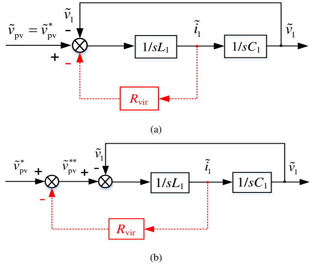
Fig. 12. Realization of the virtual resistance. (a) Original control block diagram; and (b) Equivalent transformation.
