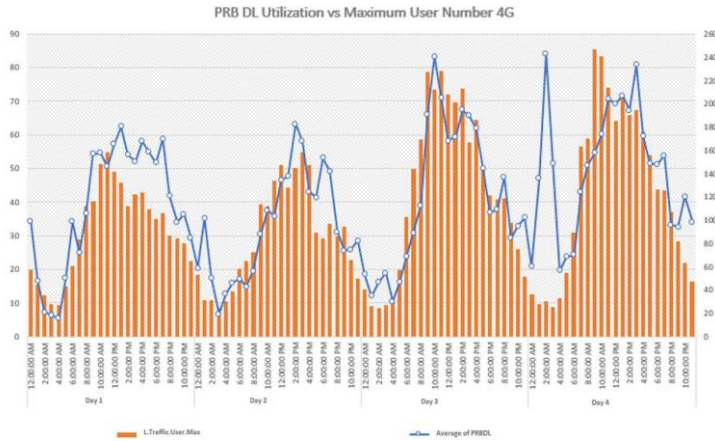
Figure 9. PRB Downlink and Number of User in 15 MHz
