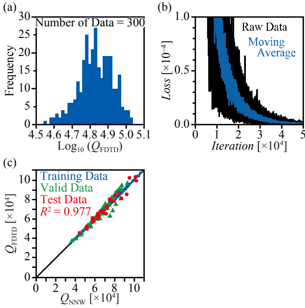
Fig. 2. The training process of NN using collected data of the Q factor. (a) Distribution of collected data. (b) Transition of error between calculated and predicted values. (c) Relation between Q calculated by FDTD and predicted by NNW.
