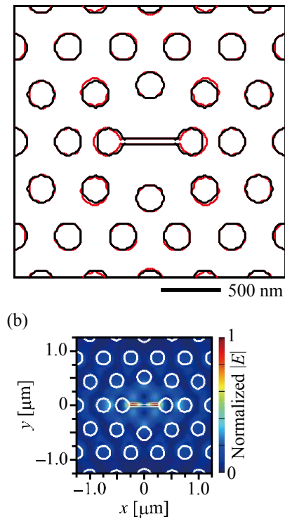
Fig. 4. H0 nanocavity with nanoslot in a solution, optimized by NN. (a) Hole positions before (black) and after (red) optimization. (b) Mode profile after the optimization.
