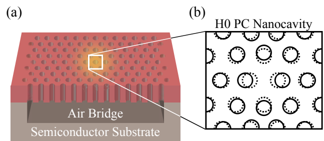
Fig. 1. Schematic of the H0 PC nanocavity. (a) Overview. (b) Magnified view of the hole arrangement around the nanocavity. The solid lines show the hole positions modified by machine learning, while the dotted lines show the original positions.
