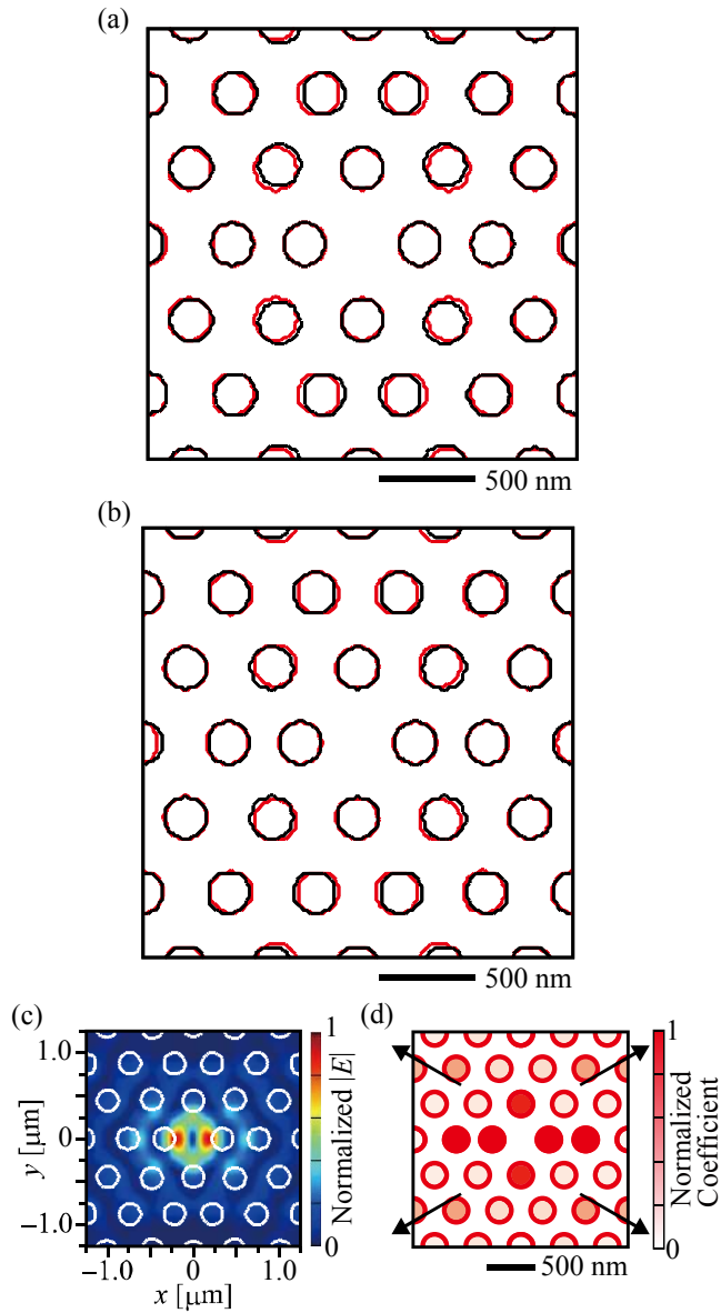
Fig. 3. The H0 nanocavity without nanoslot in a solution optimized by NN. (a), (b) The hole positions before (black) and after (red) optimization, respectively, which were obtained by using NN and Lasso regression models. (c) Mode profile after the NN optimization. (d) Visualized coefficient strength between Q and shift amount of each hole, which was estimated by the Lasso model. Four arrows indicate the directions of mode penetration.
