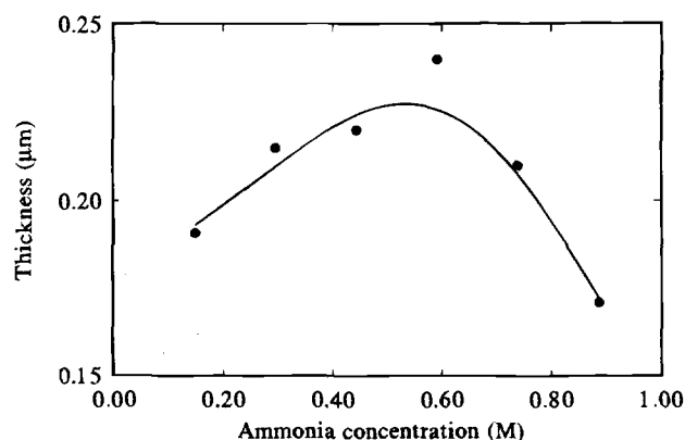
Fig. 1. Influence of ammonia concentration on CdS film thickness. Growth conditions: T = 85°C, [Cd(CH 3 COO) 2 ] = 0.002 M, [Cd(CH 3 COO) 2 ]:[SC(NH 2 ) 2 ] = 1:6, [NH 4 CH 3 COO] = 0.04 M, time of deposition 30 min.
