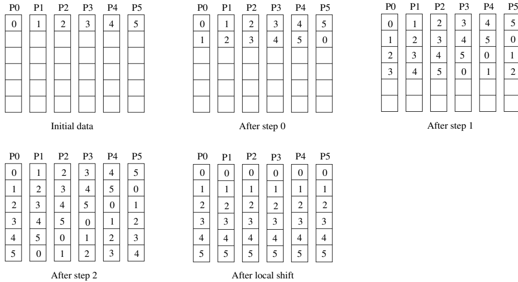
Figure 2: Bruck allgather
