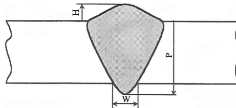
Figure 1. Bead geometry [17].
