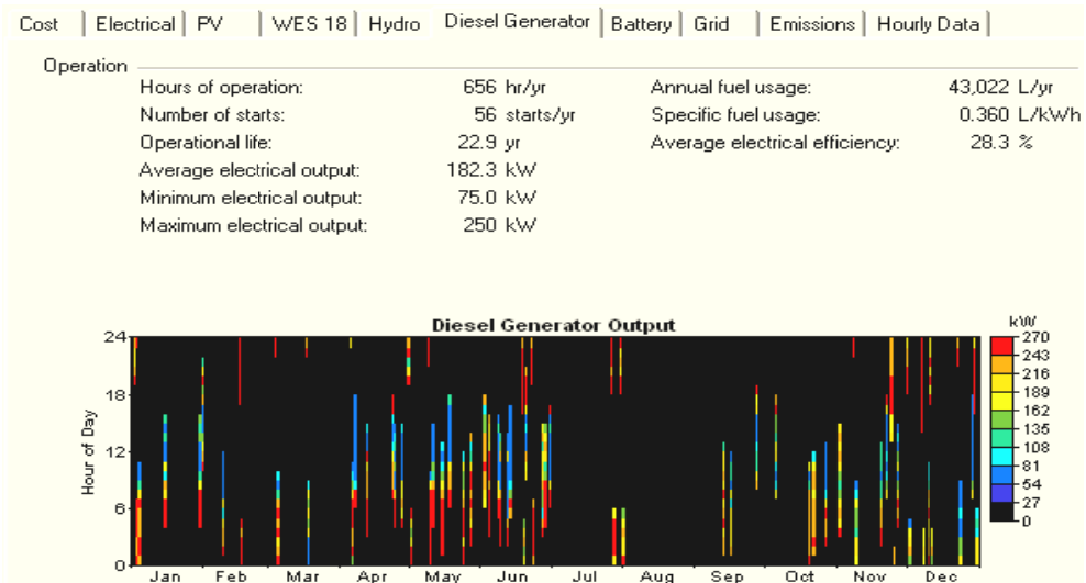
Figure 13. Annual electric production of Diesel Generator
