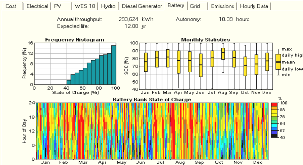
Figure16. Statistical results of battery system
