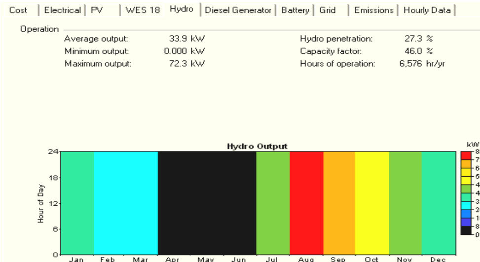
Figure15. Annual electrical energy production of hydro plant
