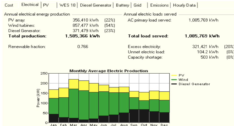
Figure19 Contribution of electrical energy production by various energy sources in the system without micro-hydro plant.
