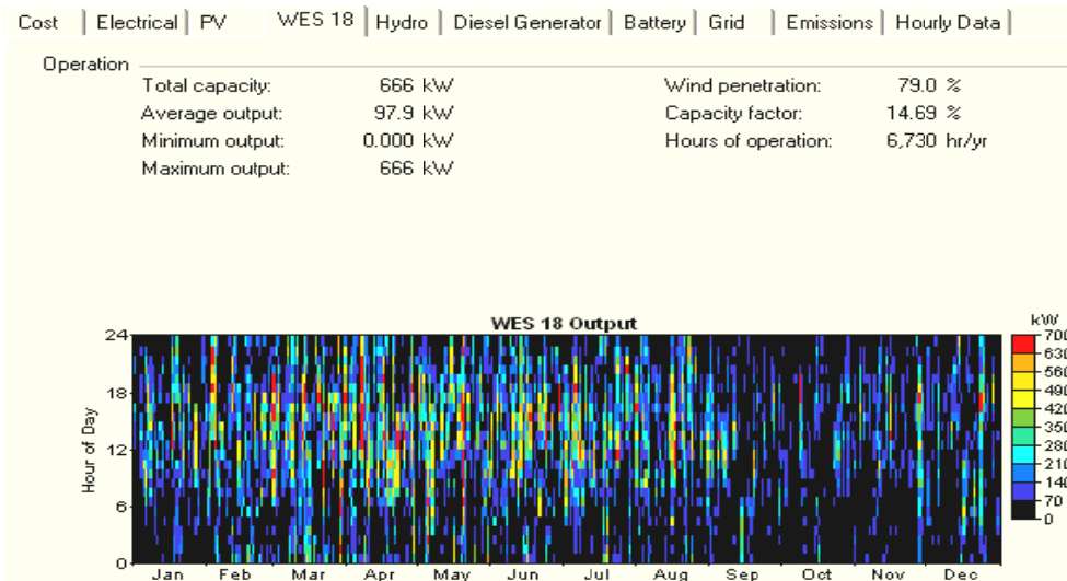
Figure 14. Annual electric production of wind energy generator
