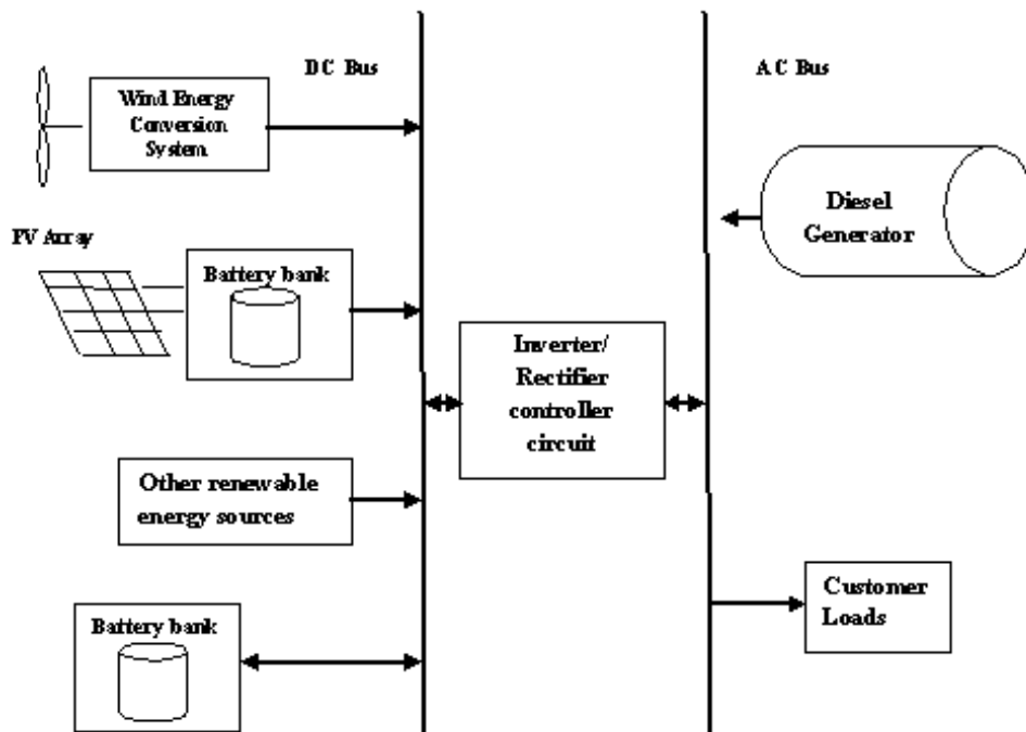
Figure 1. Parallel hybrid renewable/alternative energy system
