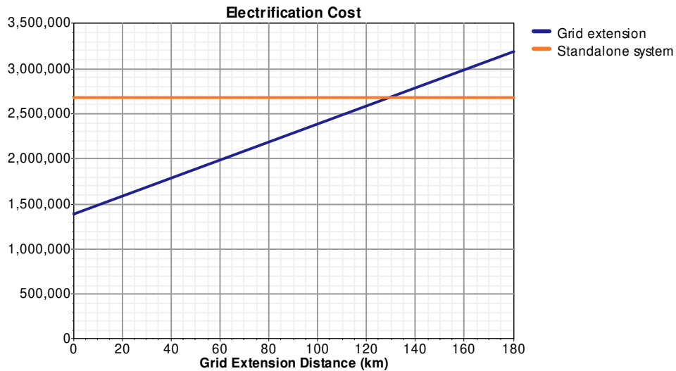
Figure17. Break-even grid distance
