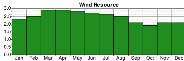
Figure 4. Monthly average wind speed
