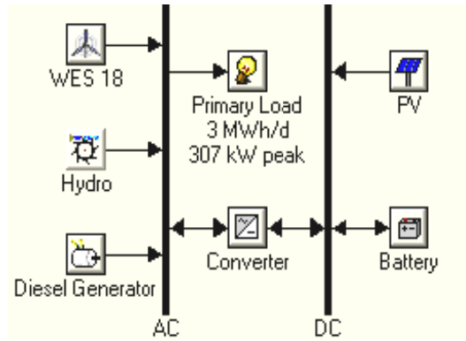
Figure 7. Proposed scheme of hybrid energy generation for the study area in HOMER software model
