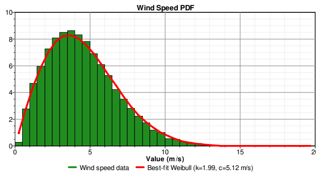
Figure 5. Wind speed probability distribution
