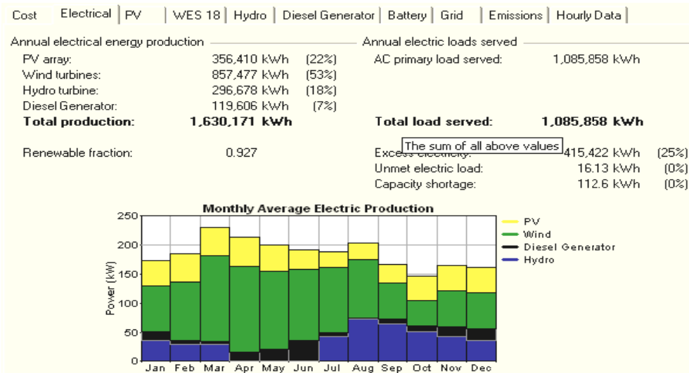
Figure 11. Contribution of electrical energy production by various energy sources in the optimal system.
