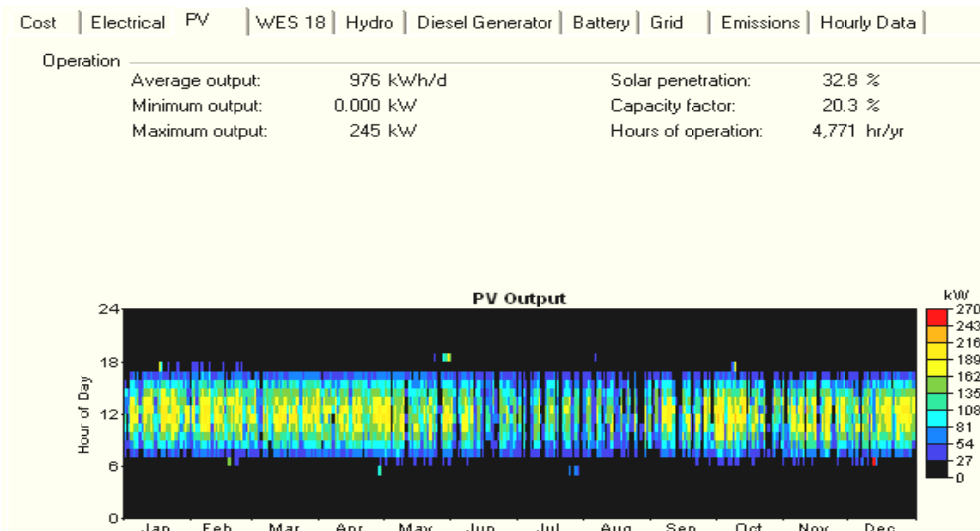
Figure 12. Annual electric production of PV system
