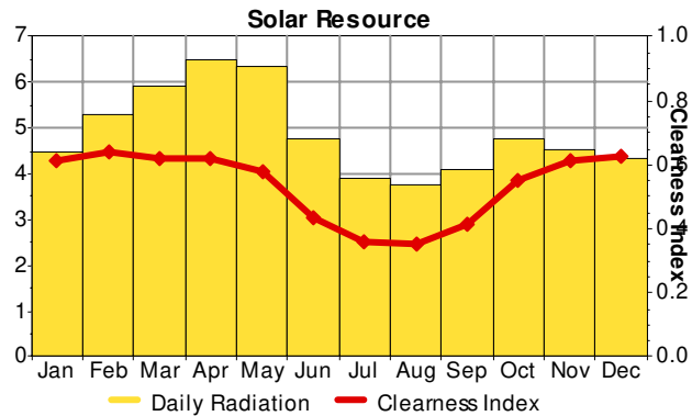
Figure 3. Monthly average daily radiation and clearness index
