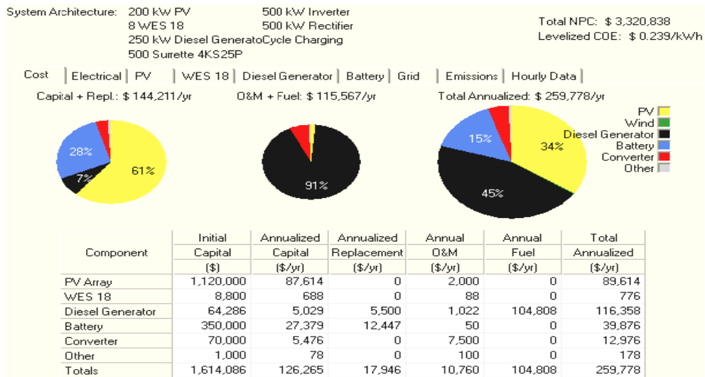
Figure18. Cost sheet of the optimum system without micro-hydro plant.
