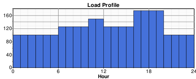
Figure 8. Hourly load consumption
