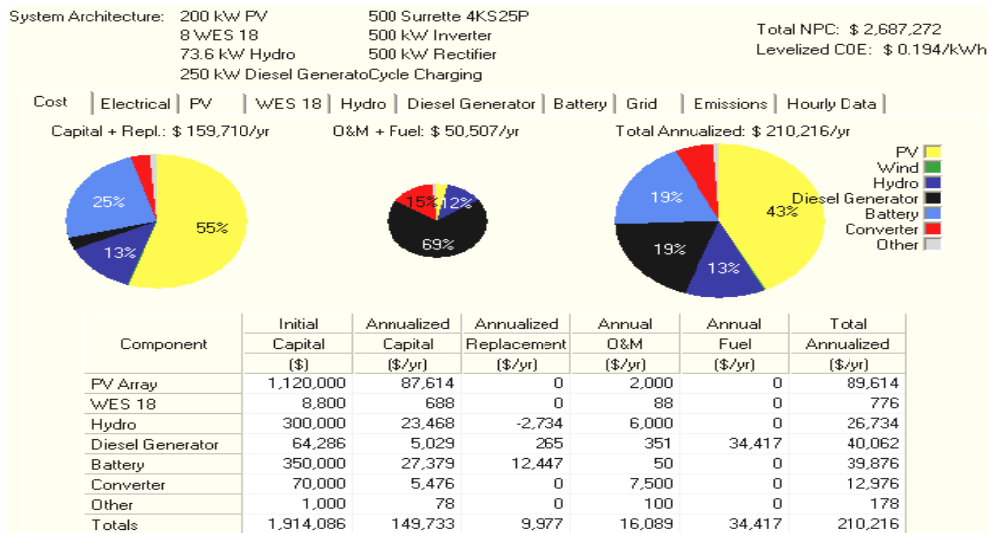
Figure 10. Cost sheet of the optimum system
