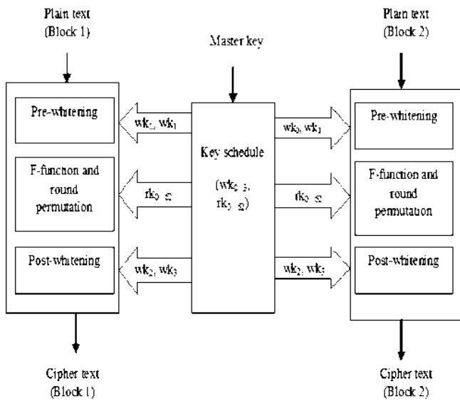
Figure 3. Novel architecture for Piccolo
