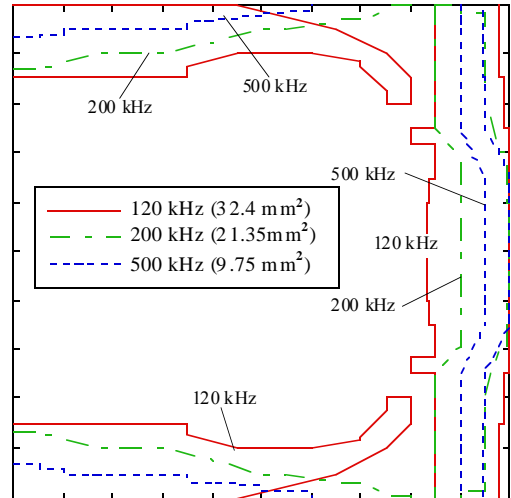
Fig. 6. Optimal winding shapes computed by COOS as in Figs. 4 and 5, but for higher frequencies. Conductors fill the indicated areas along the top and bottom walls and near the right wall.
