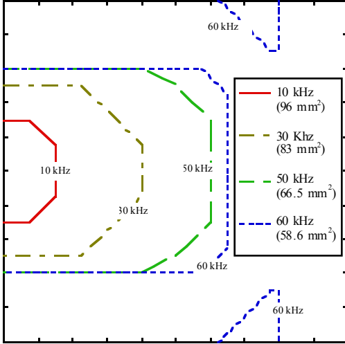
Fig. 4. Optimal winding shapes computed by COOS for a 10 mm x 10 mm winding window with a gap at the center left and 0.1 mm litz-wire strand diameter, for four frequencies. The area near the gap, bordered by the appropriate line for a given frequency, is empty of conductors. Cross-sectional area used by each solution is indicated. For the 60 kHz (58.6 mm 2 ) solution, additional empty areas appear at the top and bottom right.
