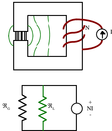
Fig. A1. Gapped inductor and corresponding magnetic circuit
