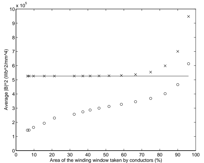
Fig. 8. Average square of magnetic field, \overline{|B|^2} , as a function of winding area for configurations based on three different design approaches. The proximity-effect loss is determined by \overline{|B|^2} , whereas the dc loss is determined by the winding area. Thus, this illustrates the design tradeoffs possible with each approach. The solid line is a rectangular winding with a distributed gap. The 'x's are designs using a rectangular winding and a lumped gap, with the winding spaced as far from the gap as possible. The circles are the optimal designs computed by COOS.
