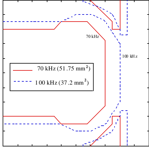
Fig. 5. Optimal winding shapes computed by COOS as in Fig. 4, but for higher frequencies. Areas empty of wire are bordered by the lines shown and include a “mushroom” shape based at the gap, bordered by the indicated line, and the wedges at the top and bottom right.
