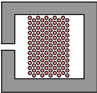
Fig. 2. Two-dimensional inductor configuration analyzed, shown with a winding that has not been optimized.
