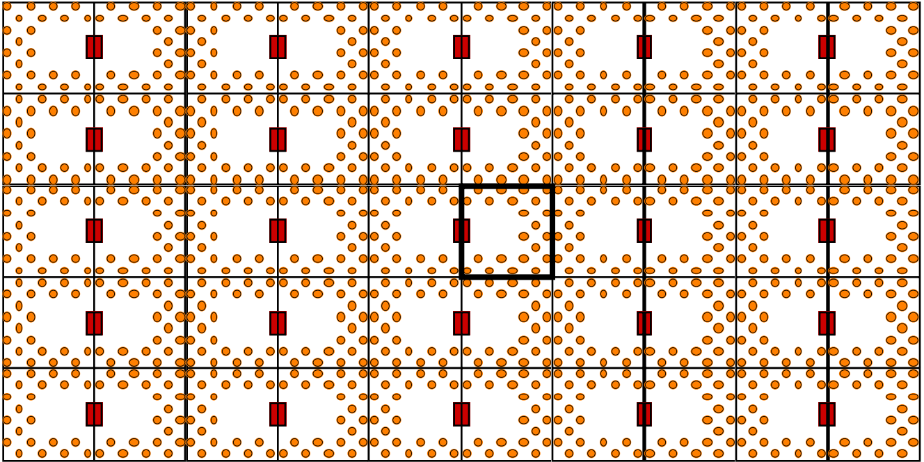
Fig. A3. Array of image currents used to calculate the field in the winding window. The original winding window near the center is outlined with a dark square, and includes round wire windings and a current representing the gap. This original with its image to the left are repeated in a 5 x 5 array of images.
