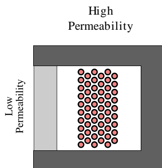
Fig. 1. Distributed-gap inductor design.
