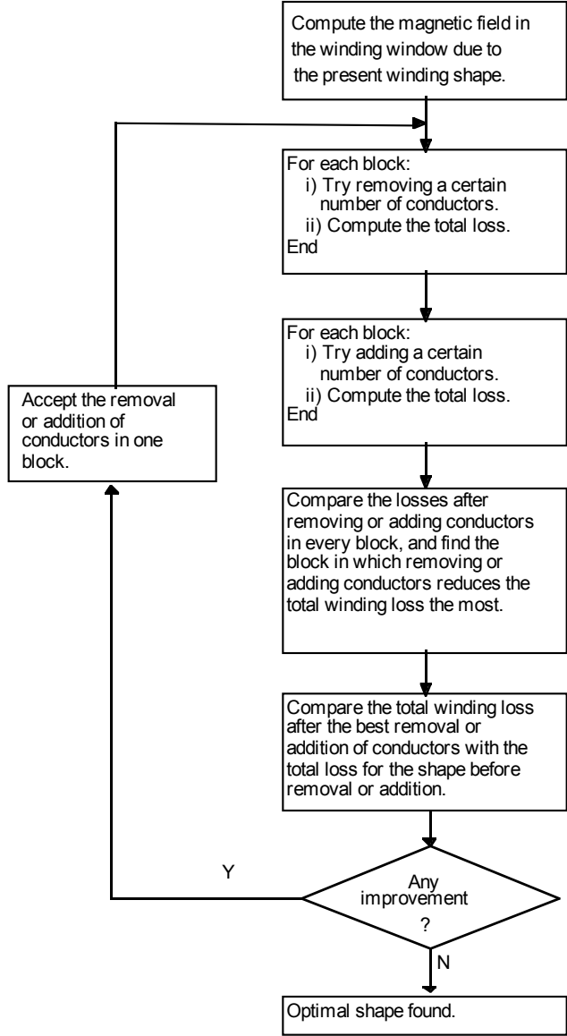
Fig. 3. Flow chart of the COOS optimization algorithm.
