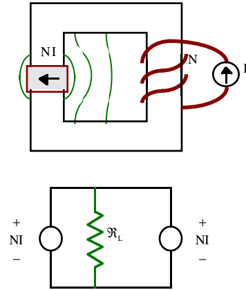
Fig. A2. Equivalent structure and corresponding magnetic circuit.
