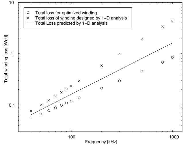
Fig. 7. Total winding loss for three different configurations. The solid line shows loss for designs optimized using one-dimensional analysis. This would be the actual loss in an optimized distributed-gap design. However, if these same designs are constructed with a lumped gap, the loss (computed by using FEA to find \overline{|B|^2} ) will be higher, as indicated by the 'x' marks on this plot. For this, we assume the winding is spaced 2 mm from a 1-mm-long gap. The circles indicate loss with designs optimized by COOS.
