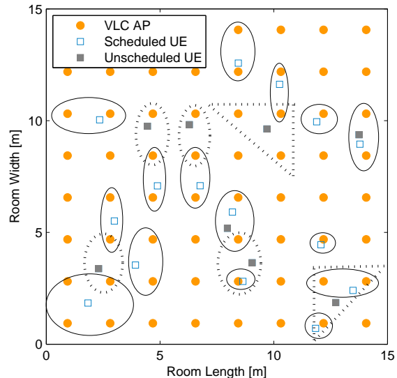
Fig. 10: The amorphous UC multi-AP clusters constructed for jointly transmitting data to a single UE by employing CT, where the multiple APs convey the same information on the same visible carrier frequency and served a single UE at a time. When multiple UEs can receive data from the same AP, only one of them can be granted access for the sake of avoiding extra interference.
