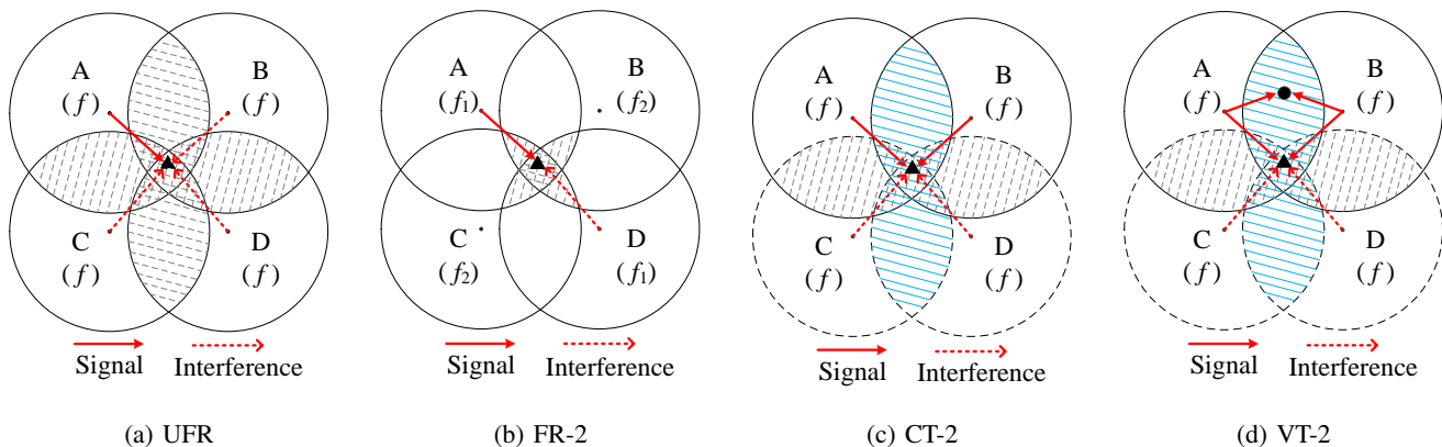
Fig. 7: Different network-centric cell formations [76]. (a) is a regular cell formation, (b) has a FR factor of two, (c) represents two merged 2-AP cells with CT and (d) shows two merged 2-AP cells using VT. The triangle and circle denote certain points of reception. The shaded areas covered with dotted lines represent the ICI imposed by the LOS ray of neighbouring cells at the cell edge. The shaded areas covered by solid lines represent the overlapping areas within the merged 2-AP cells. In (a), (c) and (d), the entire frequency band f is used by each small cell, while in (b) orthogonal frequencies f_1 and f_2 are employed by neighbouring cells, where we have f_1 = f_2 = f/2 .
