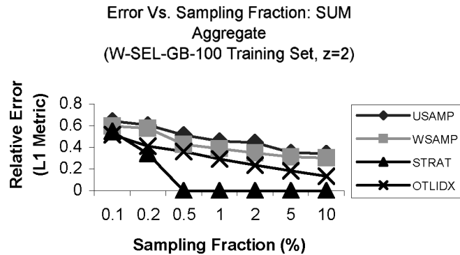
Fig. 8. SUM aggregate—training set.
