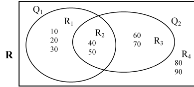
Fig. 3. Fundamental regions.
