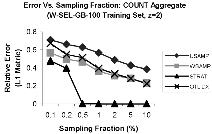
Fig. 7. COUNT aggregate—training set.
