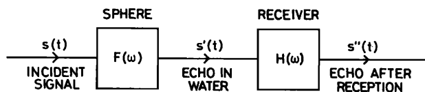
FIG. 1. Schematic diagram of acoustic backscattering as a filtering process.
