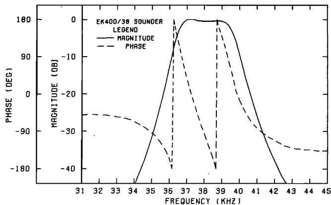
FIG. 4. Measured frequency response function of the Simrad EK-400/38 echo sounder.
