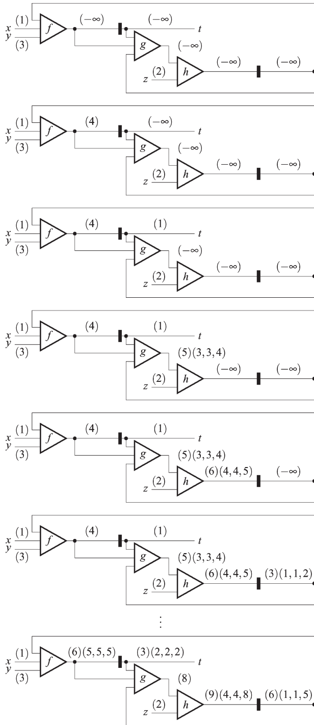
Fig. 12. Computing FATs for a circuit with desired period c = 3 . Each gate has delay 2. The topmost circuit is the initial condition; the bottom is the fixed point. A total of seven complete passes over the circuit was required to find the fixed point; only the relaxation steps taken during the first are shown.
