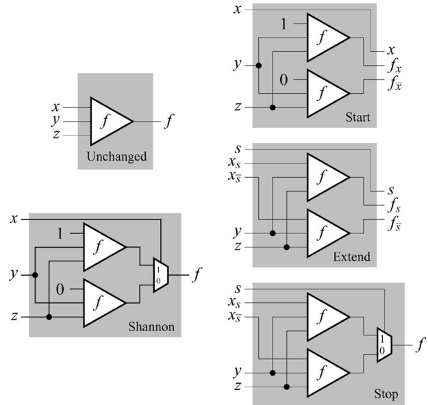
Fig. 5. Basic Shannon “cell library.”
