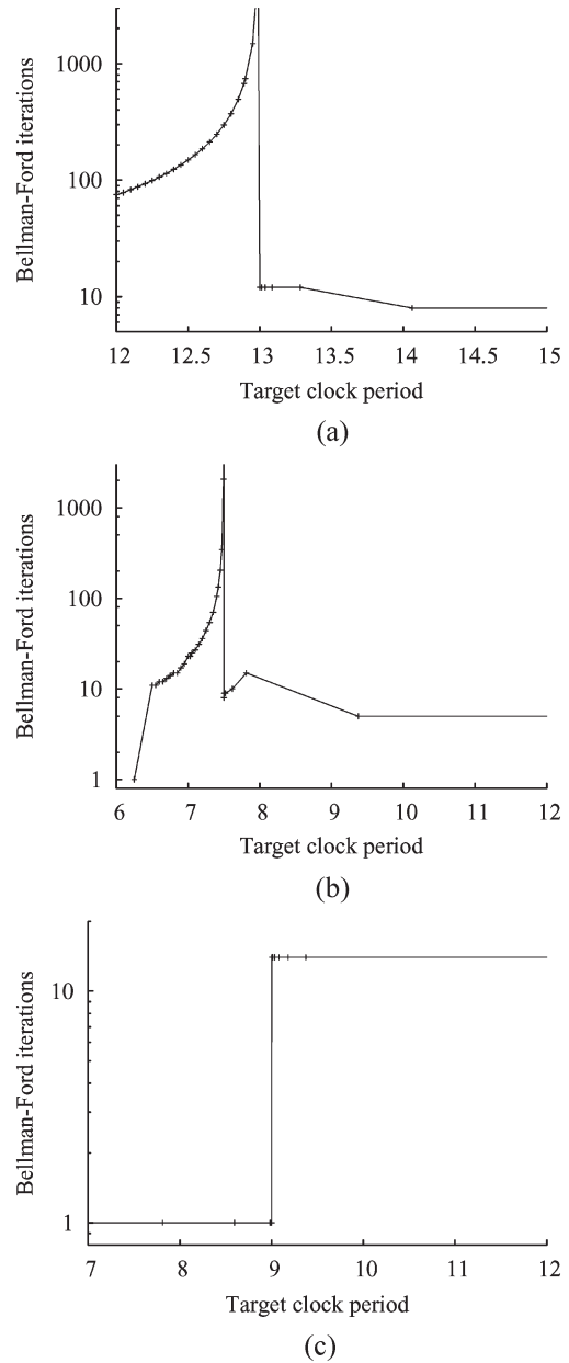
Fig. 11. Iterations near the lowest c . (a) s38417 circuit sample. (b) s9234 circuit sample. (c) s13207 circuit sample.
