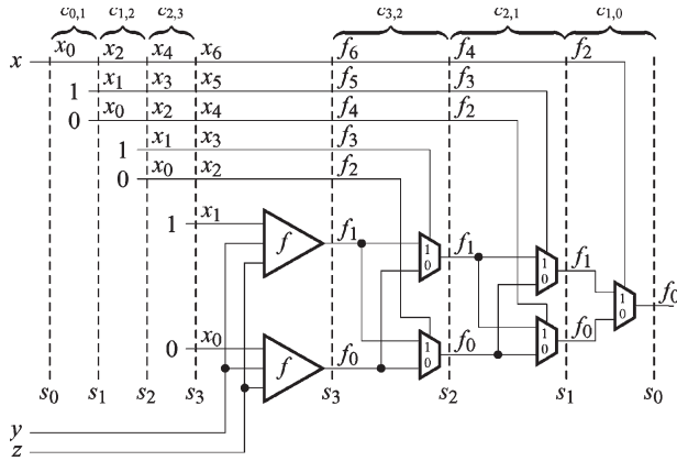
Fig. 8. Encoding x , evaluating f(x, y, z) , and decoding the output for the s_0, s_1, s_2 , and s_3 codes.
