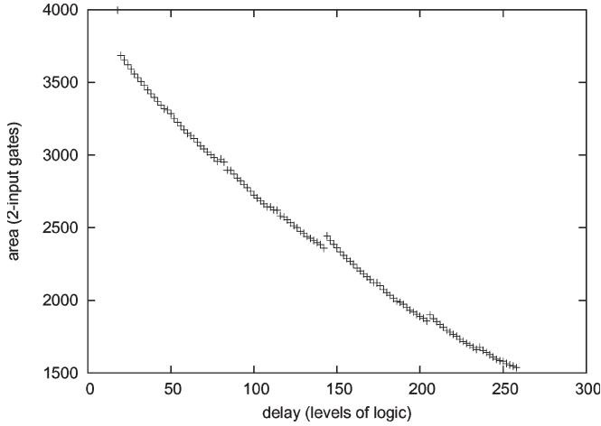
Fig. 16. Performance/area tradeoff obtained by our algorithm on a 128-bit ripple-carry adder.
