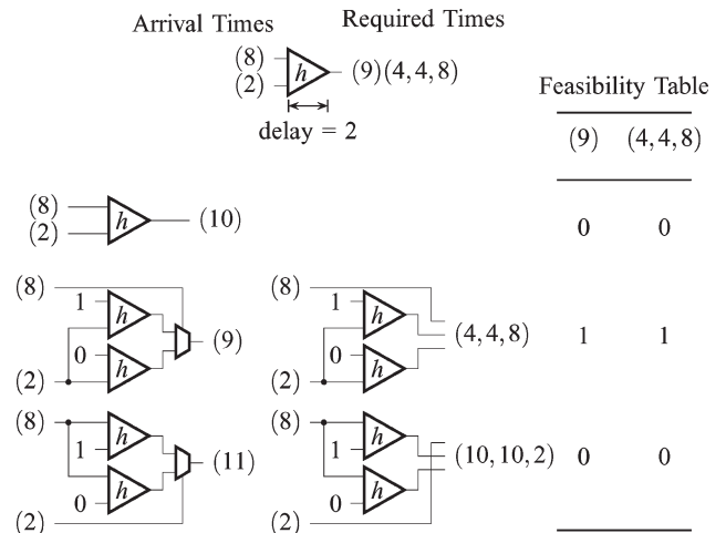
Fig. 14. Selecting cells for node h in Fig. 12.
