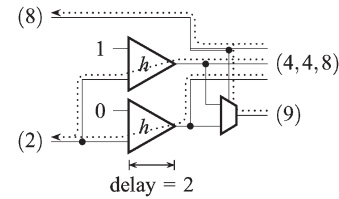
Fig. 15. Propagating required times from outputs to inputs. Only the critical paths (dotted lines) impose constraints.
