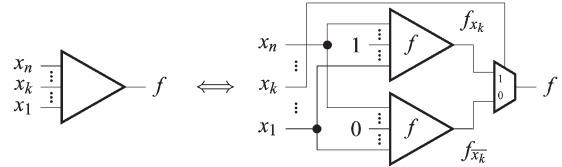
Fig. 4. Shannon decomposition of f with respect to x_k .
