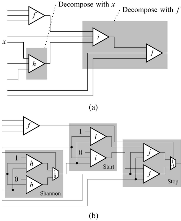
Fig. 6. Shannon decomposition through node replacement. (a) Initial circuit. (b) After Shannon transformation.
