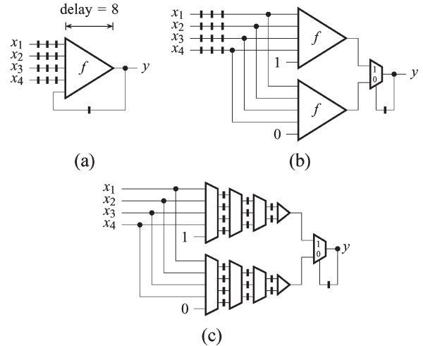
Fig. 1. (a) Single-cycle feedback loop prevents retiming from improving this circuit, but (b) applying Shannon decomposition reduces the delay around the loop so that (c) retiming can distribute registers and reduce the clock period.
