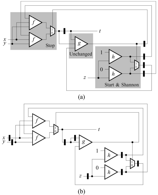
Fig. 13. (a) Circuit from Fig. 12 restructured according to the FAT sets. Its period (9) happens to be the same as that of the original; in general, it is different (and not necessarily better). (b) After retiming, the circuit runs with period 3 as desired.
