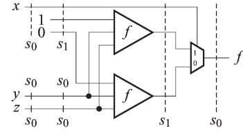
Fig. 7. Shannon transform as redundant encoding.
