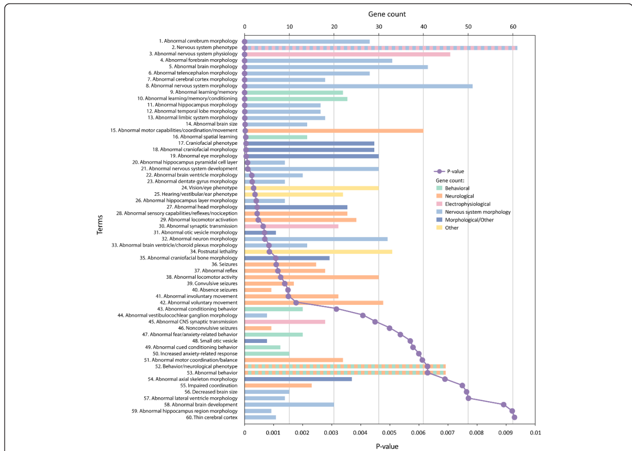
Figure 1 Mouse phenotype categories associated with ASD genes. ASD genes (n = 112) were analyzed for enrichment in mouse phenotypes using ToppGene with a Bonferroni corrected P value cutoff of 0.01. Categories are arranged from most significant and downwards (purple line), and for each category, the number of genes in the ASD112 list for which there were murine models with the associated category are indicated by the length of the horizontal bars (gene count). To highlight differing phenotypic categories discussed in the text, bars are color-coded as indicated in the inset to the figure. Categories relating to nervous system morphology phenotype domains are colored light blue, while other morphological categories are colored dark blue, electrophysiological categories are colored pink, neurological categories are colored peach, and higher-order behavioral categories are colored green. Categories corresponding to more than one phenotyping domain are presented as alternating colors, and categories that do not relate to our phenotyping scheme are colored yellow. All data are also found in tabular form in Additional file 2.
