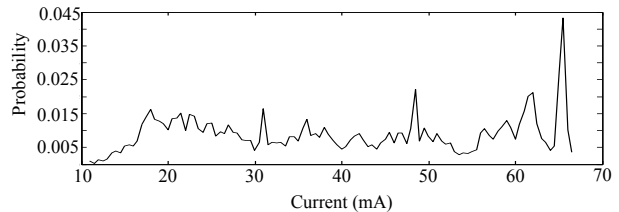
Fig. 16. Load current distribution of display modules in Group 7, according to the 10 brightness levels.
