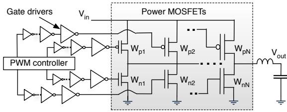
Fig. 7. Circuit diagram for dynamic switch modulation.
