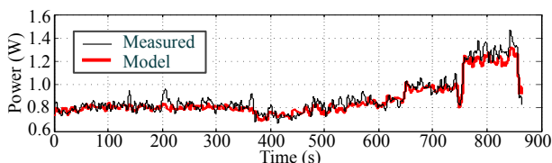
Fig. 13. A part of traces of total power consumption: measured data and modeled data.
