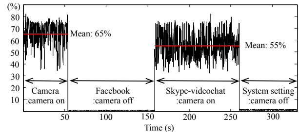
Fig. 15. The ratio of the power consumed by Camera digital to the power consumed by all the modules in Group 4.
