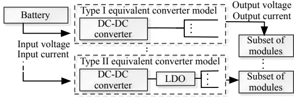
Fig. 11. Types I and II equivalent converter models.
