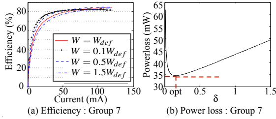
Fig. 14. Relation between the power conversion efficiency and W : Group 7
