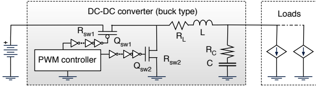
Fig. 3. Circuit diagram of a buck type inductive DC-DC converter.
