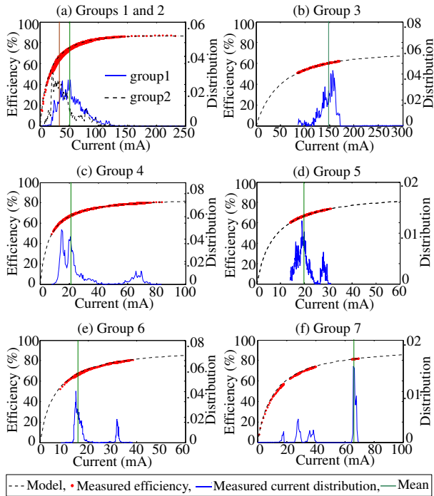
Fig. 12. Conversion efficiencies for all groups.
