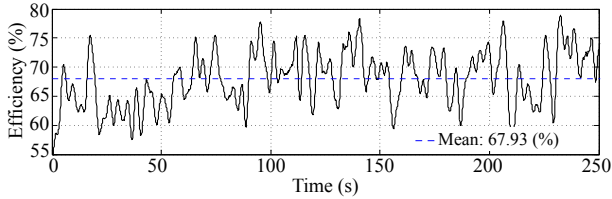
Fig. 2. Measured of traces of the power conversion efficiency of the PDN in the Qualcomm Snapdragon MDP MSM8660.
