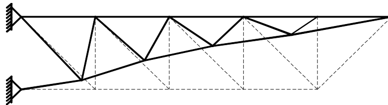
Figure 2b. Optimum layout of the 18-bar truss
