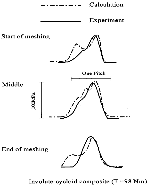
Fig. 3 Comparison of tooth root stress waveform between experimental and calculation results ( m_t=4 mm, \alpha_0=13^\circ , a=7 mm)
