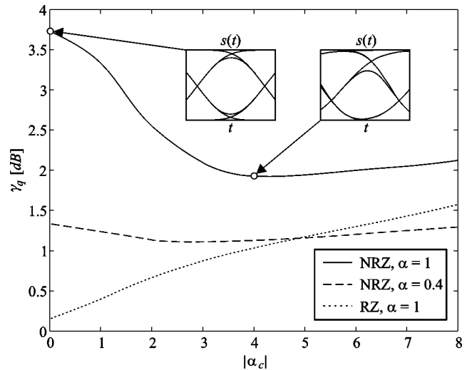
Fig. 8. Sensitivity penalty \gamma_q as a function of the chirp parameter \alpha_c for optimized FPF and BF bandwidths (solid: NRZ with \alpha = 1 , dashed: NRZ with \alpha = 0.4 , dotted: 33% duty cycle RZ with \alpha = 1 ). The better performance of chirped NRZ signals is caused by reduced (“0”-bit) ISI, as visualized by the eye diagrams.
