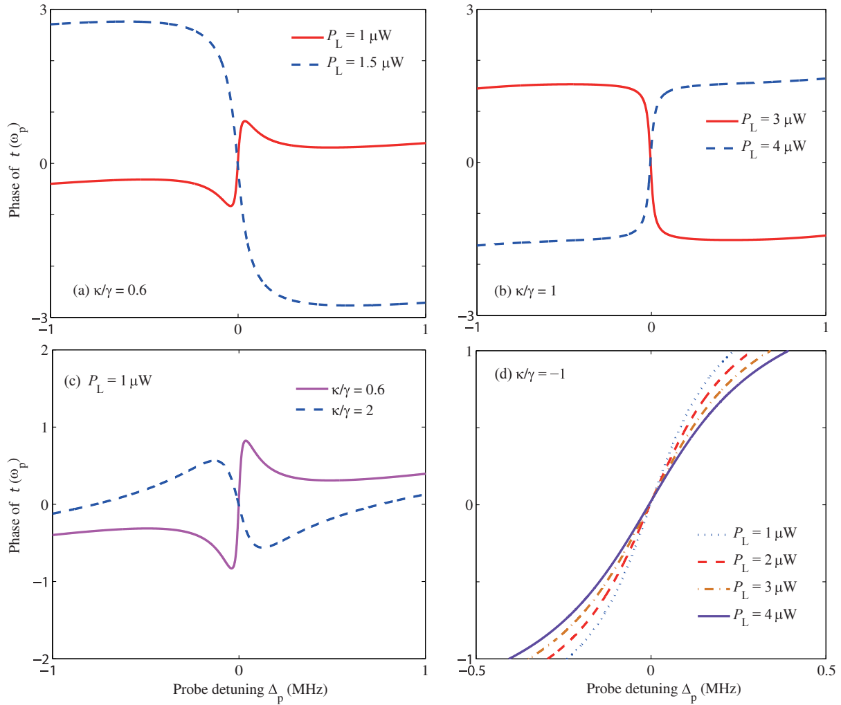
Figure 6 | The phase of the transmission amplitude t(\omega_p) with different parameters. (a–b) With different values of pump power P_L . (c) With different values of gain-to-loss ratio \kappa/\gamma . The specific values of P_L and \kappa/\gamma are taken from Fig. 5, corresponding to the slow and fast light regimes. For comparison, the results for the passive-passive COM system are also plotted in (d) with \kappa/\gamma = -1 .
