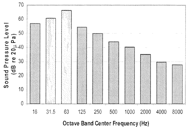
Figure 5 Frequency character of the mid-level rumble noise exposure.
