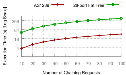
Fig. 12. Scalability of Heuristic
