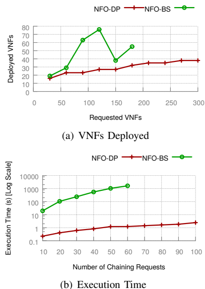
Fig. 11. Performance comparison with [14] http://www-01.ibm.com/support/docview.wss?uid=swg21399933
