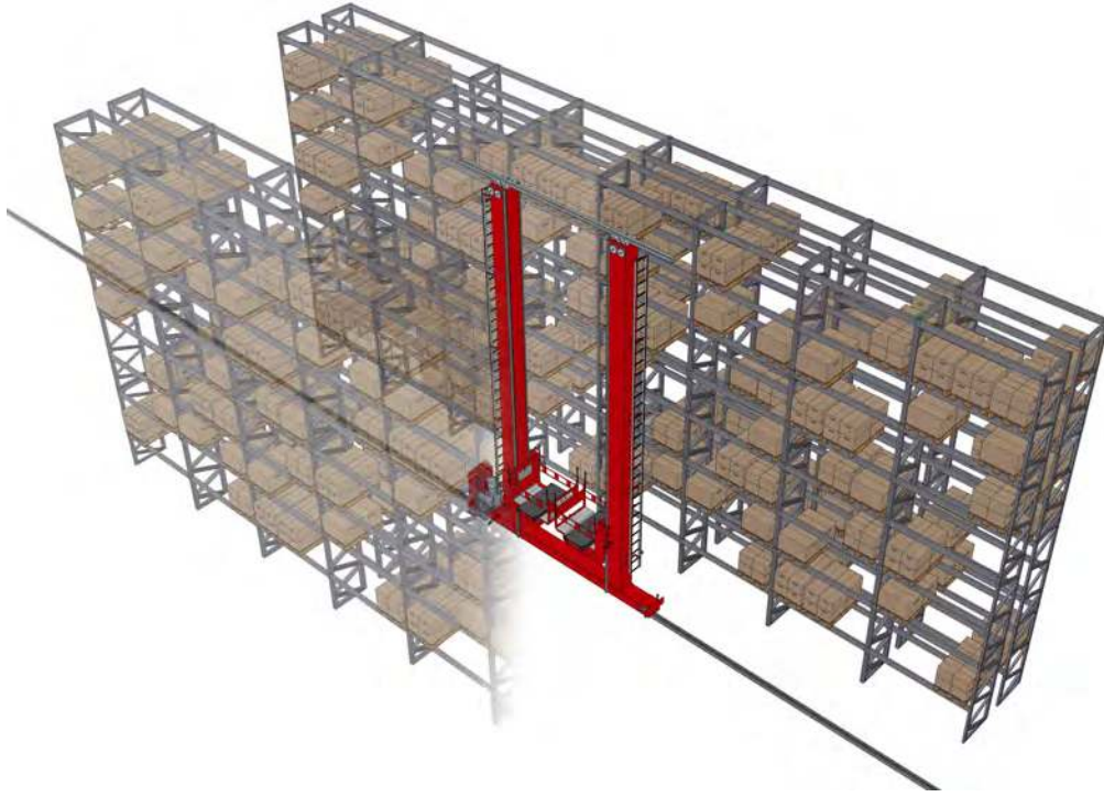
Figure 1: Schematic description of a double deep storage rack with a dual capacity AS/RS machine in the aisle
