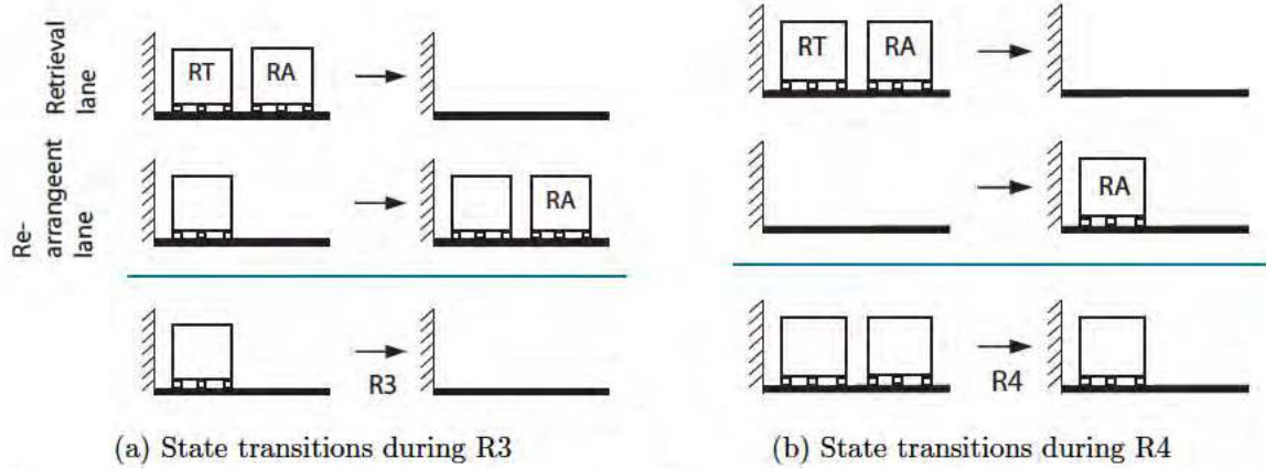
Figure 8: The two possible state transitions caused by retrieval operations with rear-arrangement
