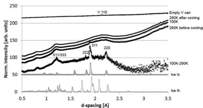
Fig. 11. Neutron diffraction pattern of Opal A1 collected with the TOF HIPPO diffractometer, 90° detector bank. Top: empty vanadium can, below TOF spectra of Opal A1 290 K after cooling, 100 K, 290 K before cooling and below a difference spectrum that displays diffraction peaks of cubic ice (scale 10 times enlarged). For comparison diffraction spectra of ideal cubic and hexagonal ice are shown at the bottom. Intensity scale is arbitrary.
